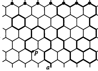
FIGURE 2. A configuration \gamma on a finite domain, with the weighted vertices on the top boundary indicated. The contribution of \gamma to F(p) is e^{-5i\sigma\pi/3}x^{51}y^3n^2 .
