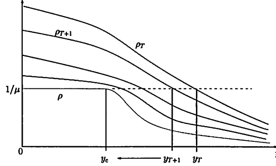
FIGURE 10. An illustration of Corollary 8.
