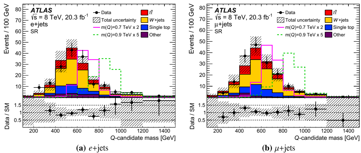
Fig. 4 Distribution of the Q -candidate mass for the electron and muon channels before the likelihood fit. The signal yields are shown for cross-sections corresponding to c_L^{Wb} = 1 and for \text{BR}(Q \rightarrow Wb) = 0.5 . These
