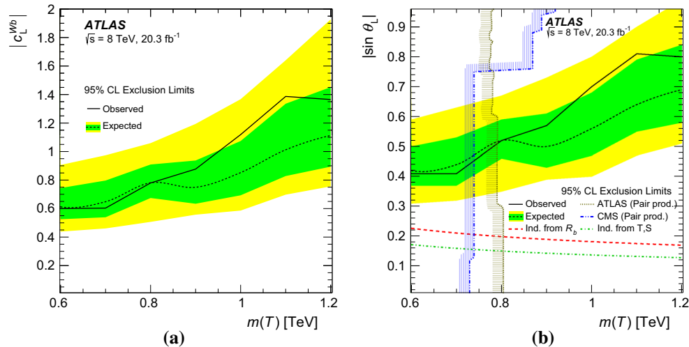
Fig. 7 a Observed and expected limit (95 % CL) on the coupling of the vector-like quark to the SM W boson and b -quark as a function of the Q mass, where the \text{BR}(T \rightarrow Wb) is assumed to be 50 %. The excluded region is given by the area above the solid black line . b Observed and expected limit (95 % CL) on the mixing of a singlet vector-like T quark to the SM sector, where the \text{BR}(T \rightarrow Wb) is assumed to be that of a sin-
