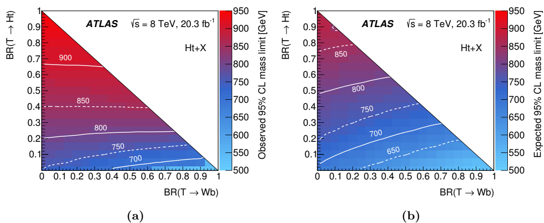
Figure 33. (a) Observed and (b) expected limit (95% CL) on the mass of the T quark in the plane of BR(T \rightarrow Ht) versus BR(T \rightarrow Wb) for the T\bar{T} \rightarrow Ht+X search. Contour lines are provided to guide the eye.
