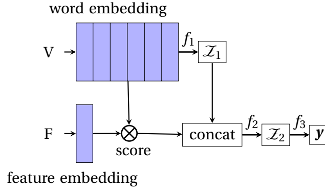
Figure 4.2 Illustration of our proposed method (Feature-guided). Here: \otimes denotes cosine similarity between the feature indicator and word embeddings; f_1 and f_2 denote Bi-LSTM layers; f_3 denotes a dense layer; \mathcal{Z}_1 and \mathcal{Z}_2 denote sentence and document representations, respectively; V and F are the document input and feature indicators, respectively; and y is the target output.
