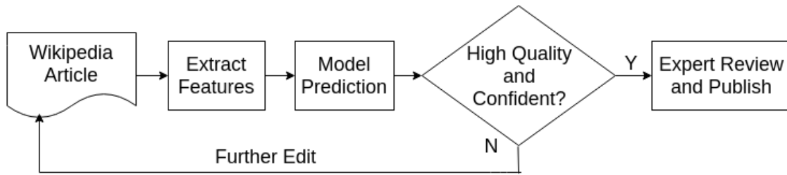
Figure 5.2 Model application and decision-making procedure.
