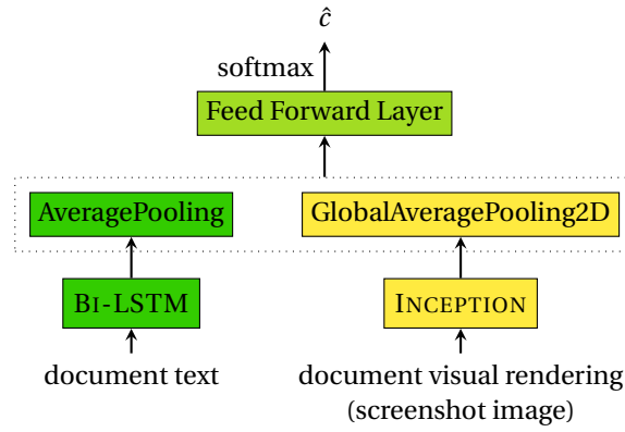
Figure 3.3 Illustration of our proposed model (JOINT), which consists of textual and visual models.
