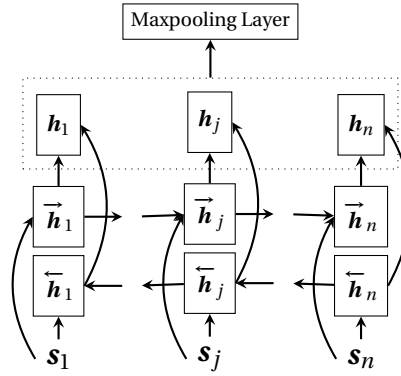
Figure 3.2 Illustration of the textual model (B1-LSTM), a component of our JOINT model.
