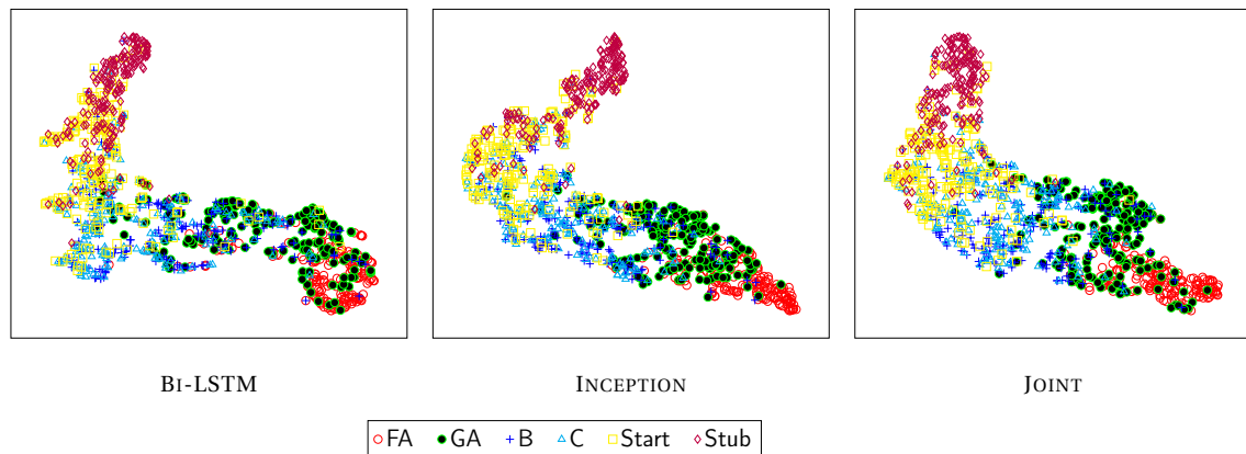
Figure 3.5 t-SNE scatter plot of Wikipedia article representations (representations from the penultimate layer of each model, based on 200 random samples from each quality class; best viewed in colour).
