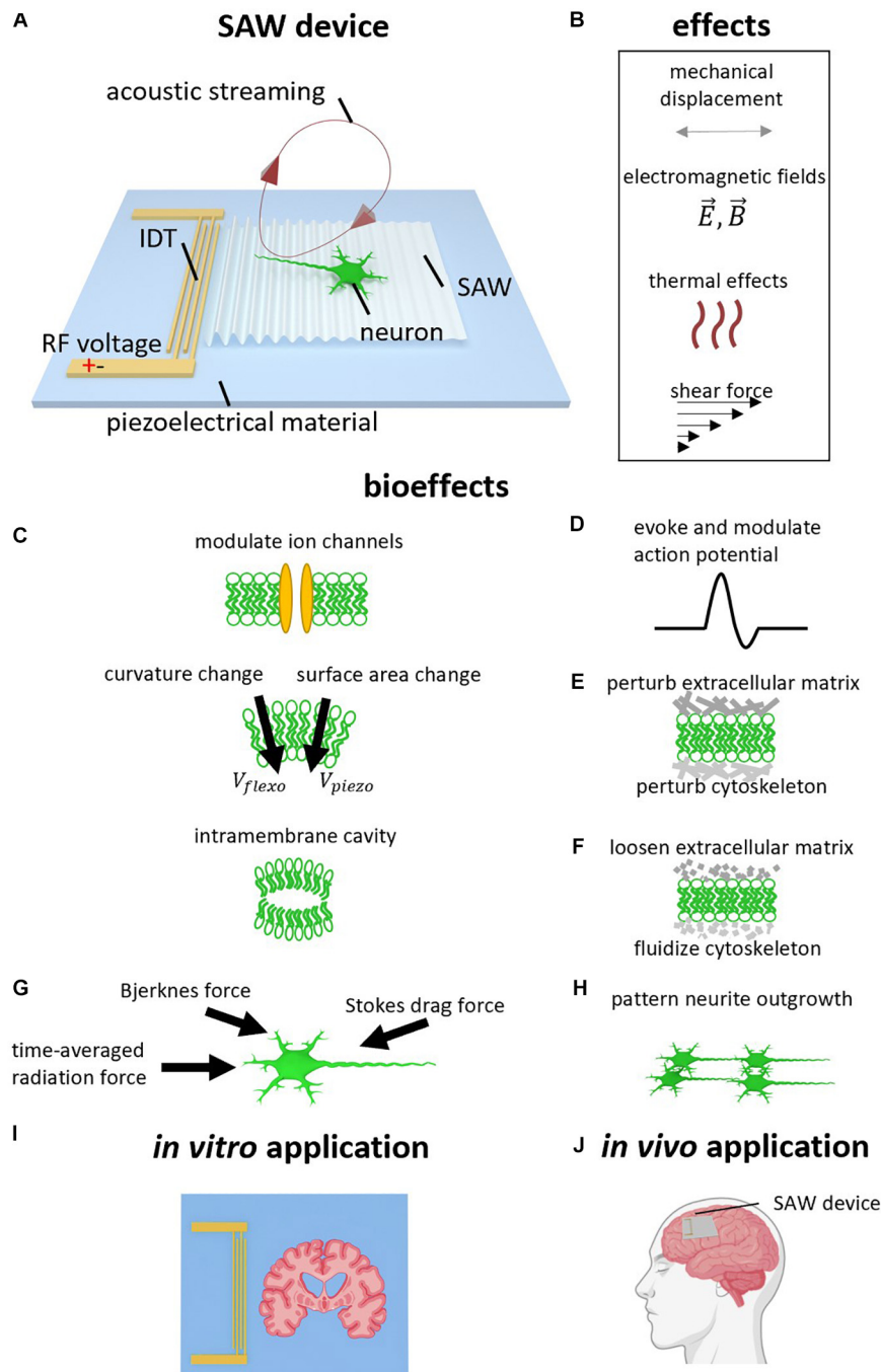
FIGURE 1 | Surface acoustic wave (SAW) neurostimulation mechanisms. (A) SAW device. Radio frequency AC voltage is applied to the interdigital transducer (IDT) to generate a SAW which propagates on the surface of the piezoelectric substrate. The SAW refracts the longitudinal wave into the neural medium at the Rayleigh angle. The refracted longitudinal wave results in acoustic streaming. (B) Acoustic effects caused by SAW device. In addition to the acoustic vibration, other effects due to the high frequency electromagnetic field, heating, and shear forces may also be considered. (B–H) Bioeffects caused by acoustic effects. (C) Ion channels can be modulated, and the generated ultrasound can change membrane curvature, surface area, and generate intramembrane cavities. (D) Action Potentials (AP) can therefore be evoked and modulated. (E) The ultrasound can perturb the extracellular matrix and cytoskeleton. (F) Ultrasound can also loosen the extracellular matrix and fluidize the cytoskeleton, analogous to the rejuvenation of soft glassy materials. (G) SAW actuation generates acoustic forces including the acoustic radiation force, intercellular Bjerknes force, and the Stokes drag force. (H) Neurite outgrowth can be patterned via SAW. (I) In vitro application using SAW device to stimulate brain slice. (J) Potential In vivo application using wearable or implantable SAW device to treat neurological disorder.
