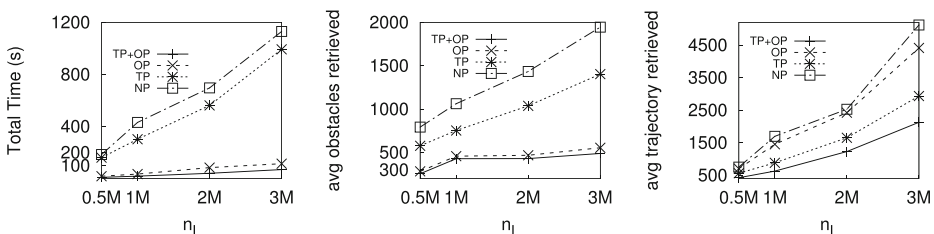
Fig. 17 Effect of n_L in Boston downtown dataset
