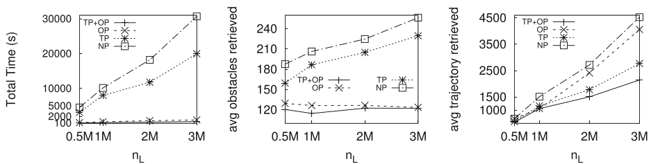
Fig. 18 Effect of n_L in Synthetic dataset
