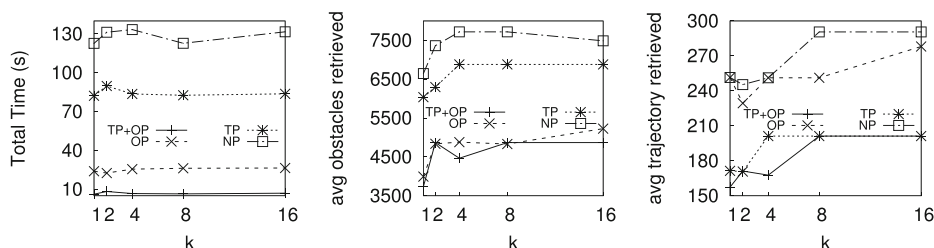
Fig. 11 Effect of k in New York dataset
