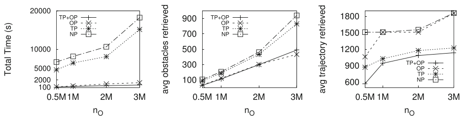
Fig. 19 Effect of n_O in Synthetic dataset
