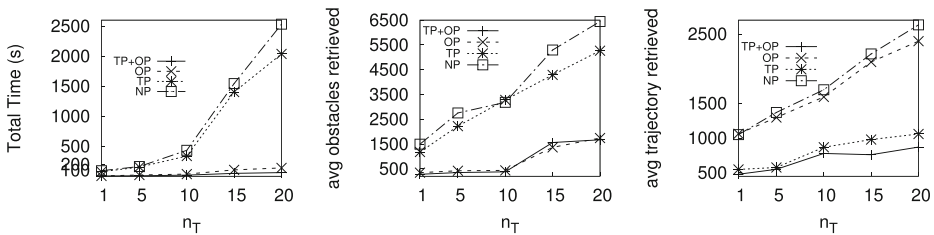
Fig. 16 Effect of n_T (BN dataset)
