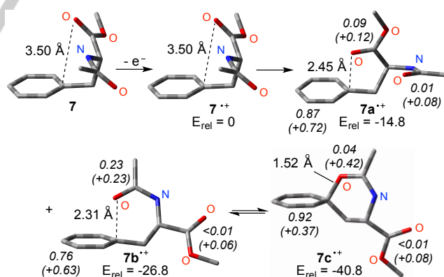
Scheme 4. Stabilization of the arene radical cation of phenylalanine 7 by neighbouring group participation. Energies E_{\text{rel}} in kJ mol -1 (in acetonitrile) relative to 7 •+ , which retains the conformation of neutral 7 (see Table S1). Italic numbers: spin densities and increases in Mulliken atomic charges from 7 (in brackets) summed up for the phenyl ring and the amide/ester moieties.
