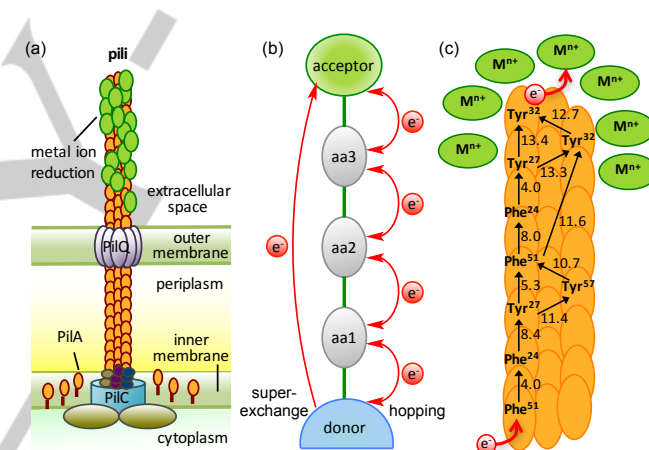
Figure 1. a) Extracellular electron transfer (EET) from respiration sites at the inner cell membrane to metal ions outside the cell during mineral respiration uses conductive protein filaments (pili). b) ET through peptides can proceed through a coherent tunnelling process (superexchange) or through a hopping mechanism using side chains of amino acids (aa1-3) as stepping stones. c) Pili transport electrons using Tyr and Phe as relay amino acids. Orange "footballs" are peptides that aggregate to the pili. Interaromatic distances in Å for the Asp2 pilus (cell constituents are omitted for clarity). [12]
