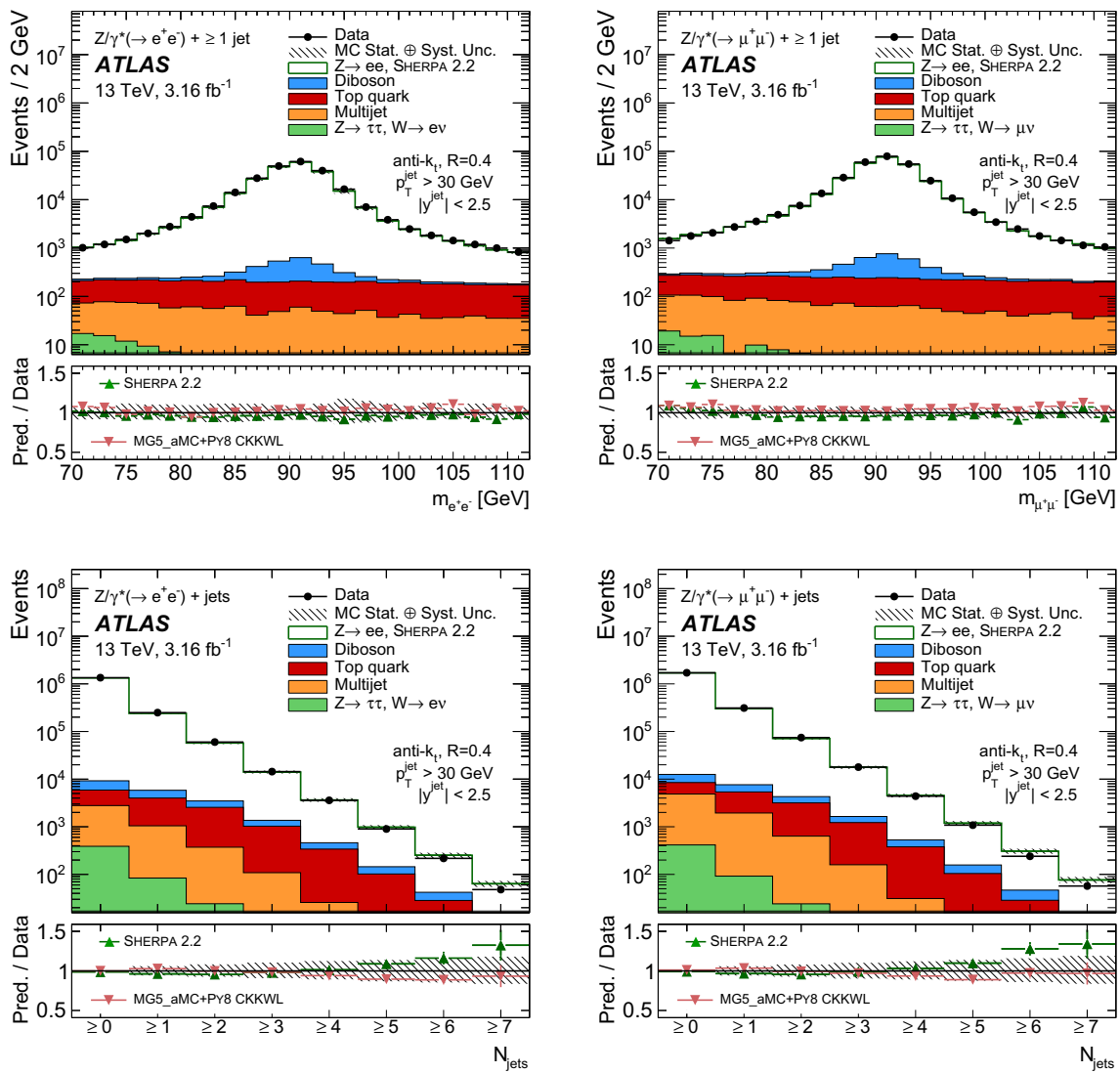
Fig. 1 Dilepton invariant mass for Z + \geq 1 jet (top) and inclusive jet multiplicity (bottom) in the Z(\rightarrow e^+e^-) + jets (left) and the Z(\rightarrow \mu^+\mu^-) + jets (right) channels. All backgrounds and the signal samples are stacked to produce the figures. Systematic uncertainties
