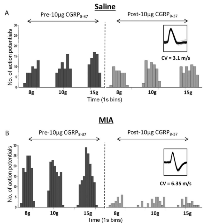
Figure 2. Inhibition of knee afferent mechanical evoked firing by the calcitonin gene-related peptide (CGRP) receptor antagonist CGRP 8–37 in monosodium iodoacetate (MIA)-treated rats. Representative examples of knee afferent mechanical evoked (8-, 10-, or 15-gm von Frey monofilaments) response data recorded before and after administration of 10 \mu\text{g} of CGRP 8–37 in a saline-treated rat (A) and an MIA-treated rat (B) are shown. The inhibitory effects of CGRP 8–37 were more pronounced following MIA treatment. Results are represented as rate histograms (1-second bins) of action potential firing of knee afferents (single units) in response to stimulation at the indicated von Frey monofilament level. Insets show an overlay of a representative fiber recording with the corresponding conduction velocity (CV; in meters/second), demonstrating single-fiber recordings; both are A \delta fibers.
