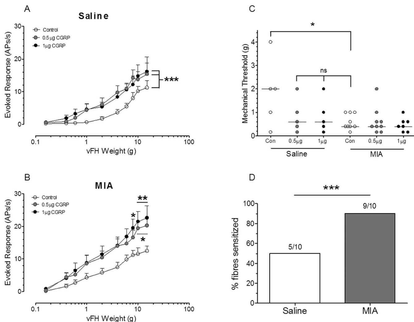
Figure 1. Calcitonin gene-related peptide (CGRP)-induced mechanical sensitization of an increased proportion of knee afferents following monosodium iodoacetate (MIA) injection. A and B , CGRP significantly increased the mechanical evoked firing rates (action potentials per second [APs/s]) of joint afferents in saline-treated ( A ) and MIA-treated ( B ) rats ( P < 0.001 by 2-way analysis of variance with Bonferroni post hoc test). Values are the mean \pm SEM maximum sensitizing effects of CGRP over each 1-hour recording period ( n = 9 MIA-treated rats; n = 5 saline-treated rats). C , CGRP administration reduced mechanical thresholds (minimum stimulus evoking \geq 2 action potentials) in saline-treated rats to a level not significantly different from that in MIA-treated rats ( P > 0.05 for comparisons of 0.5 \mu\text{g} or 10 \mu\text{g} of CGRP versus controls, by Mann-Whitney t -test). Mechanical thresholds in MIA-treated rats were unaltered by CGRP administration. Each circle represents an individual rat ( n = 7 – 9 MIA treated and n = 5 saline treated); horizontal lines show the median. D , The percentage of fibers sensitized by CGRP was greater in MIA-treated rats than in saline-treated rats ( P < 0.001 by Fisher's exact test). * = P < 0.05 ; ** = P < 0.01 ; *** = P < 0.001 by Mann-Whitney t -test. vFH = von Frey hair; NS = not significant.
