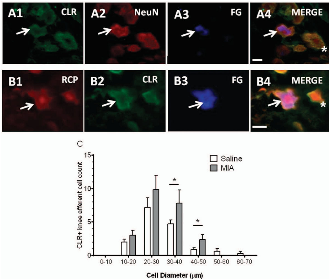
Figure 5. Coexpression of the calcitonin gene-related peptide (CGRP) receptor components calcitonin-like receptor (CLR) and receptor component protein (CRCP [RCP]) by knee afferent neurons and increased CLR expression following treatment with monosodium iodoacetate (MIA). A1–A4 , CLR is expressed on knee afferents (arrows) and non-knee afferent neuronal cell bodies (*) in ipsilateral L4 dorsal root ganglia (DRGs). Slides incubated with anti-neuronal nuclei (anti-NeuN) antibodies or with Fluoro-Gold (FG) are also shown. Bar = 34 μm. B1–B4 , CRCP is coexpressed with CLR on knee afferent neurons (arrows) and non-knee afferent neurons (*). Bar = 40 μm. C , The numbers of medium (30–40 μm in diameter) and large (40–50 μm in diameter) CLR-positive knee afferents were significantly increased in MIA-treated rats. CLR-positive knee afferent cell counts were analyzed according to diameter ranges similar to those described in a previously published report (9). Values are the mean ± SEM of 7 rats per group. * = P < 0.05 by Mann-Whitney t -test.
