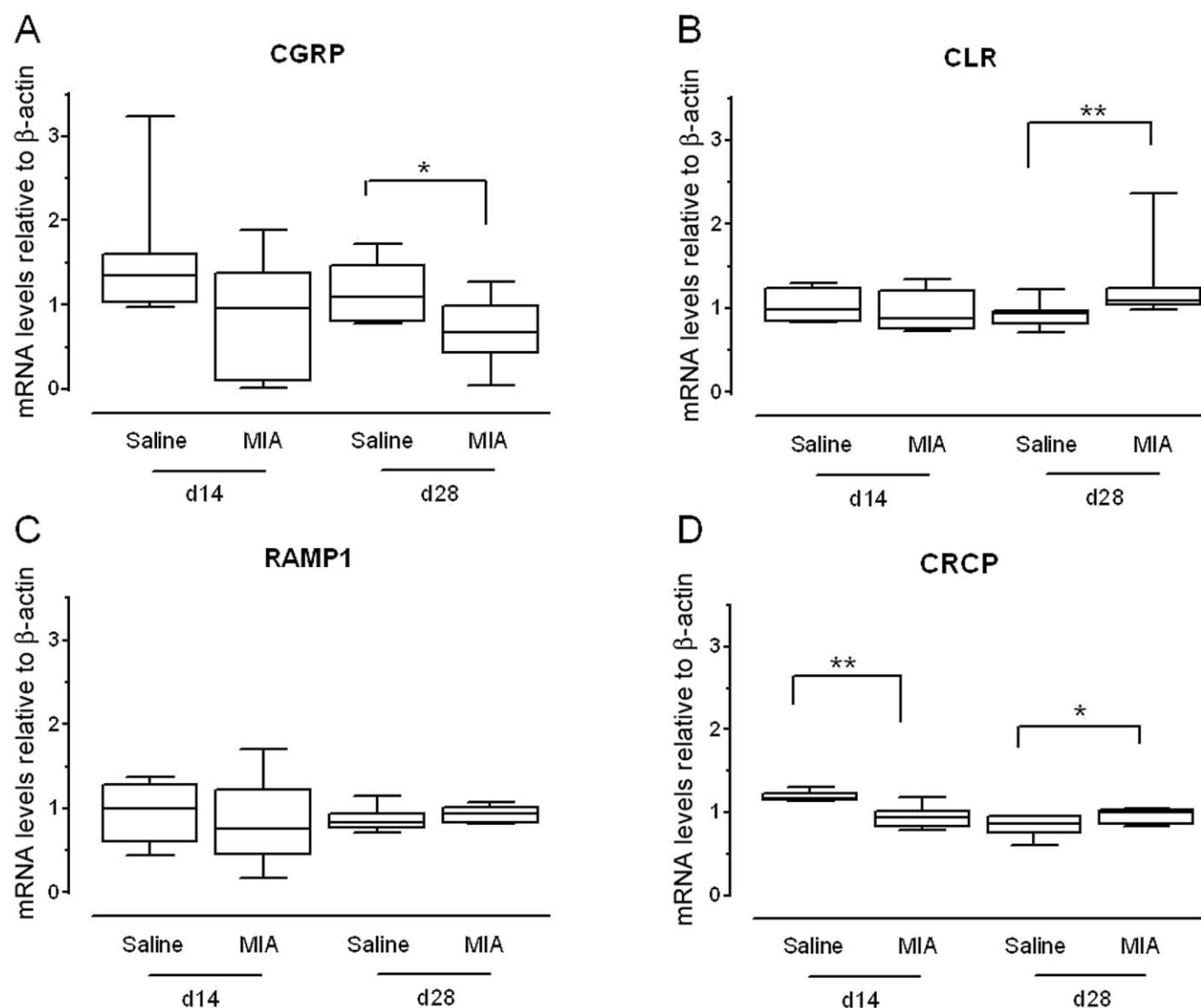
Figure 4. Expression of mRNA for calcitonin gene-related peptide (CGRP) receptor components in knee joint-innervating L3-L4 dorsal root ganglia (DRGs) and modulation of the levels following treatment with monosodium iodoacetate (MIA). A , Expression of mRNA for CGRP was significantly reduced 28 days after MIA treatment. B , Calcitonin-like receptor (CLR) expression was increased 28 days after MIA treatment. C , Levels of receptor activity-modifying protein 1 (RAMP-1) were unaltered, both on day 14 and on day 28 after MIA treatment. D , Levels of mRNA for CGRP receptor component protein (CRCP) were reduced 14 days after MIA treatment. There was a small but significant increase in CRCP expression 28 days after MIA treatment. Results were normalized to \beta -actin expression (which was unchanged between groups and treatments). Data are shown as box plots. Each box represents the 25th to 75th percentiles ( n = 6-8 rats per group). Lines inside the boxes represent the median. Lines outside the boxes represent the 10th and 90th percentiles. * = P < 0.05 ; ** = P < 0.01 by Mann-Whitney t -test.
