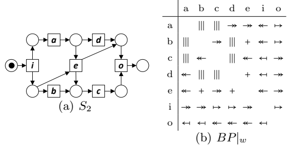
Fig. 3. Net system S_2 and its BP|_w
