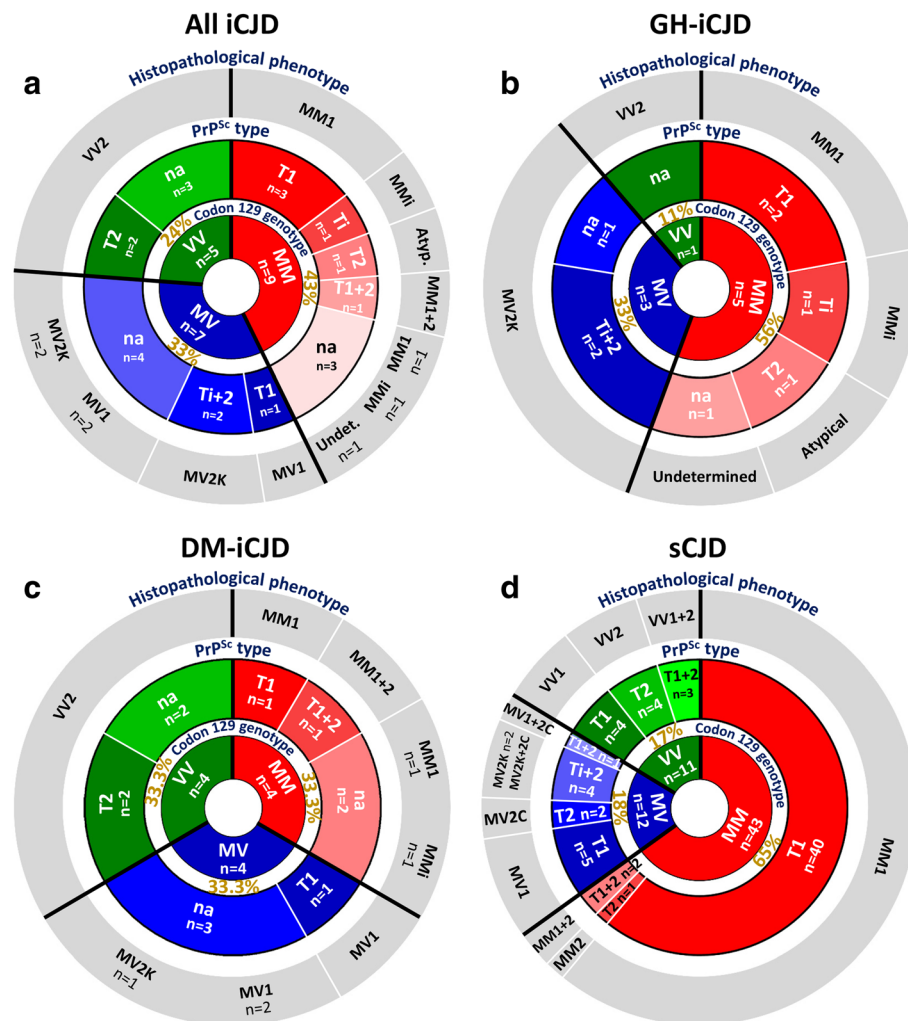
Fig. 1 Ring doughnut charts visualizing distributions of codon 129 genotypes, resPrP Sc types and disease phenotypes among iCJD and sCJD cases examined. a whole iCJD cohort; inner circle: percent distribution of codon 129 genotype (MM, MV, VV); intermediate circle: distribution of resPrP Sc types (T1, T2, Ti, T1 + 2, T1 + 2); outer circle: distribution of histopathological phenotype. b GH-iCJD, legend as a ; c DM-iCJD, legend as a ; d sCJD. T1: type 1; Ti: type intermediate; T2: type 2; T1 + 2: type 1 + 2; T1 + 2: type 1 + 2; n: number of cases; na: not available; Atyp.: atypical; Undet.: undetermined. Percentages refer to the distribution of codon 129 genotype
