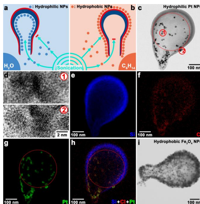
Figure 2. a, b) Selective loading hydrophilic NPs on the interior surface and hydrophobic NPs on the exterior surface of the chemically asymmetric silica NBs. c) TEM image of hydrophilic Pt NPs loaded in the cavity of Janus silica NBs. d) High-resolution TEM images of Pt NPs loaded inside the NBs (1) and adsorbed on the outer surface of the NBs (2). e-h) Elemental mapping profiles of the Pt NPs@NBs shown in c). i) TEM image of hydrophobic \text{Fe}_3\text{O}_4 NPs adsorbed on the hydrophobic exterior surface of the NBs.
