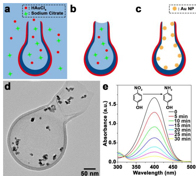
Figure 4. Chemically asymmetric silica NBs used as nanoreactors. a-c) Schematic illustration of the in situ preparation of Au NPs in the chemically asymmetric NBs. a) Dispersion of silica NBs in a solution containing HAuCl 4 and sodium citrate. b) Removal of the excess solution by centrifugation with a Millipore centrifuge tube. c) Reduction of HAuCl 4 to Au NPs in 24 h. d) TEM image of Au NPs in situ prepared in the chemically asymmetric NBs. e) UV-Vis spectra of 4-nitrophenol catalytically reduced by Au NPs@NBs nanoreactors.
