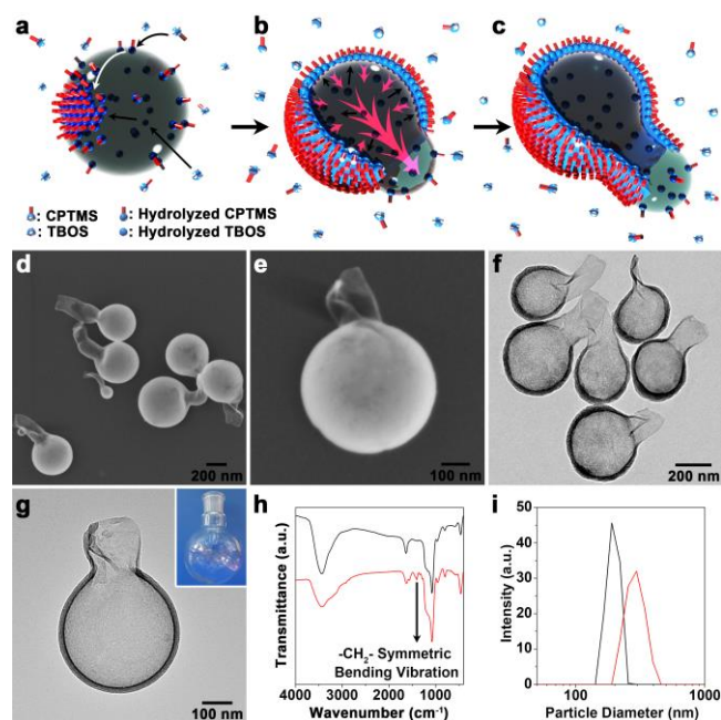
Figure 1. a-c) Schematic illustration of the formation of chemically asymmetric silica NBs. a) Hydrolyzed CPTMS arranged at the water-oil interface with hydrolyzed TBOS condensed at the interface from the water side. b) The formation of a hybrid silica shell from the co-condensation of CPTMS and TBOS; the continuous deposition of TBOS extrudes water out of the shell to form a new water-oil interface. c) The co-condensation of CPTMS and TBOS at the newly formed water-oil interface caused the formation of chemically asymmetric NBs. d, e) SEM images and f, g) TEM images of the silica NBs. h) FTIR spectra of the NBs before (red line) and after (black line) removal of organic residues. i) DLS measurement of particle size distribution of the as-prepared NBs (black line) and NBs after removal of the hydrophobic capping organic groups (red line).
