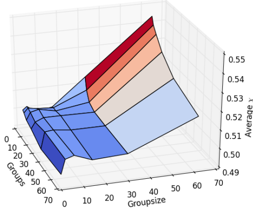
Average \chi over varying groups and groupsizes with mpcr=0.75
