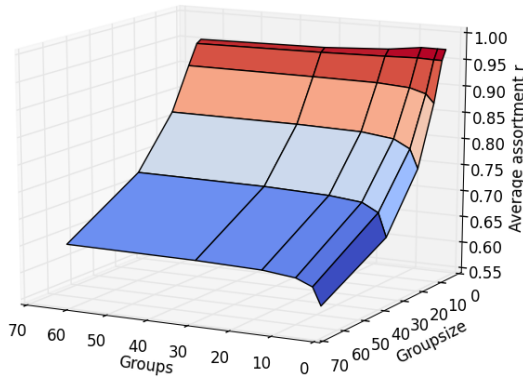
Average r over varying groups and groupsizes with mpcr=0.75
