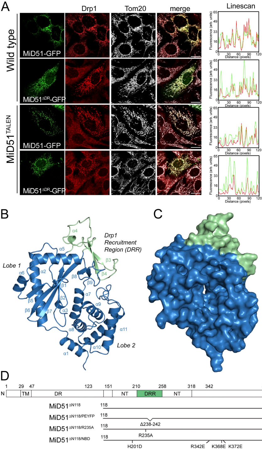
Figure 1. Crystal structure of a MiD51 cytosolic domain sufficient for Drp1 recruitment. (A) MiD51-GFP and MiD51 ΔDR -GFP were expressed in wild-type MEFs and MEFs lacking endogenous MiD51 (MiD51 TALEN ). Cells were subsequently immunostained for Drp1 and the mitochondrial marker protein Tom20 and visualized by fluorescence microscopy. (right) Linescans demonstrating colocalization of Drp1 with MiD51-GFP and MiD51 ΔDR -GFP. Bars, 20 μm. (B) Structure of MiD51 ΔN118 displaying the nucleotidyltransferase domain in blue and DRR domain in green. (C) Surface representation of MiD51 ΔN118 ; view and coloring as in B. (D) Topology of MiD51 and illustration of mutant constructs used in this study. TM, transmembrane domain; DR, disordered region; NT, nucleotidyltransferase domain.
