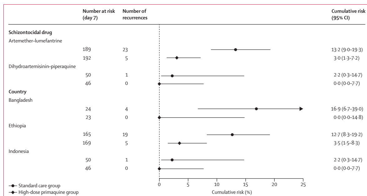
Figure 3: Risk of P vivax after P falciparum malaria at day 63 by schizontocidal drug and study site
