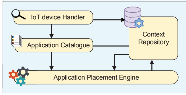
Figure 5.2: Software architecture of Fog Gateways
