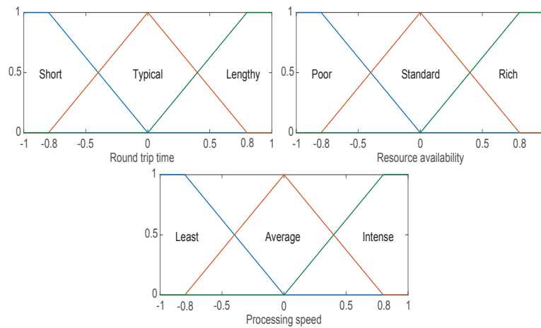
Figure 6.7: Membership function for status parameters
