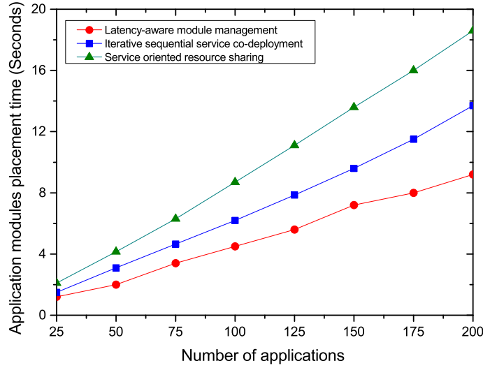
Figure 4.4: Module deployment time for varying number of applications
