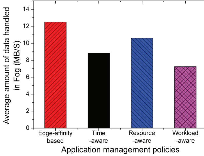
Figure 3.6: Average amount of data handled by different management policies
