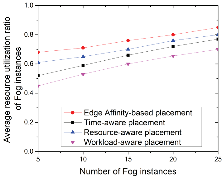
Figure 3.13: Average resource utilization for varying number of Fog instances
