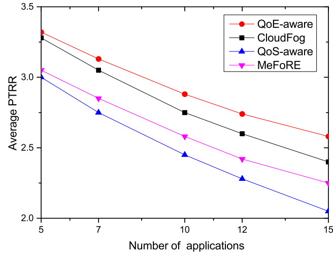
Figure 6.12: Processing time reduction for varying number of applications
