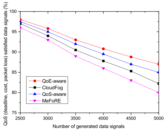
Figure 6.14: Percentage of QoS satisfaction
