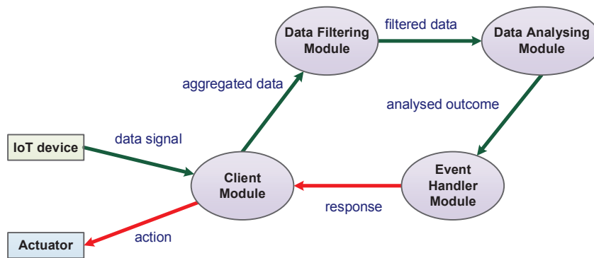
Figure 4.1: Dataflow model for a distributed application
