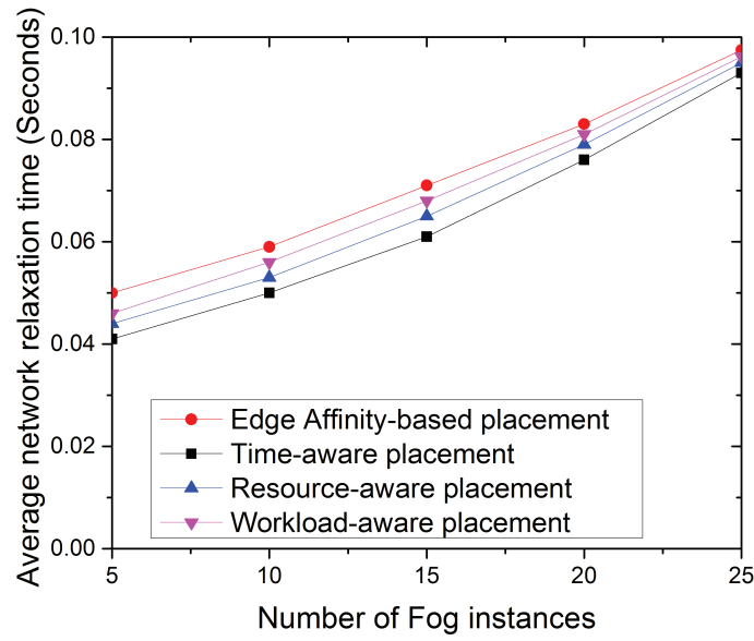
Figure 3.12: Average network relaxation for varying number of Fog instances
