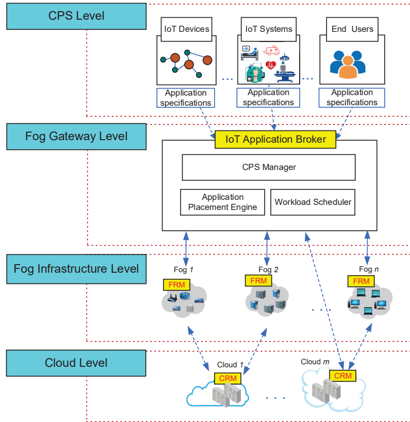
Figure 2.7: A perspective model for application management in Fog
