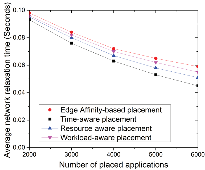
Figure 3.9: Average network relaxation for varying number of placed applications
