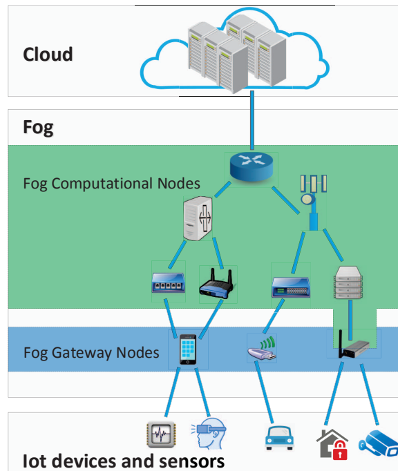
Figure 6.1: Organization of Fog environments
