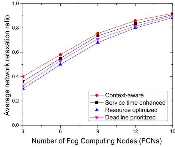
Figure 5.9: Average network relaxation for varying number of Fog nodes
