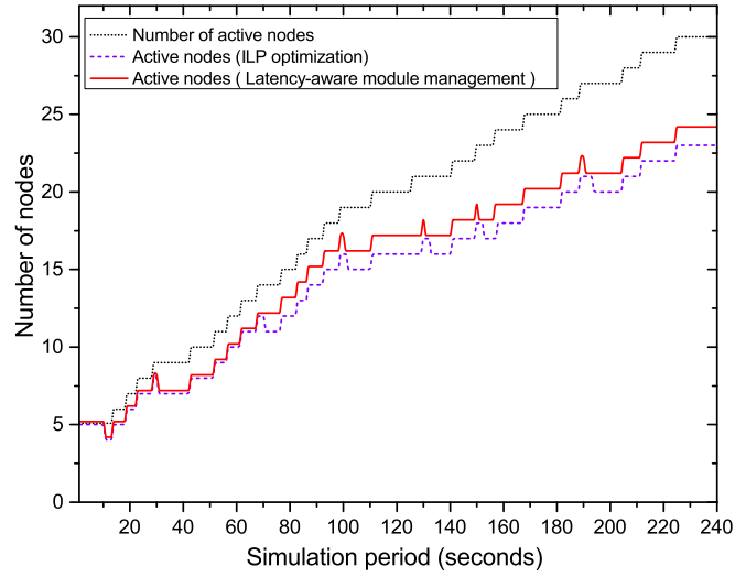
Figure 4.6: Comparison of ILP and heuristic based latency-aware solution
