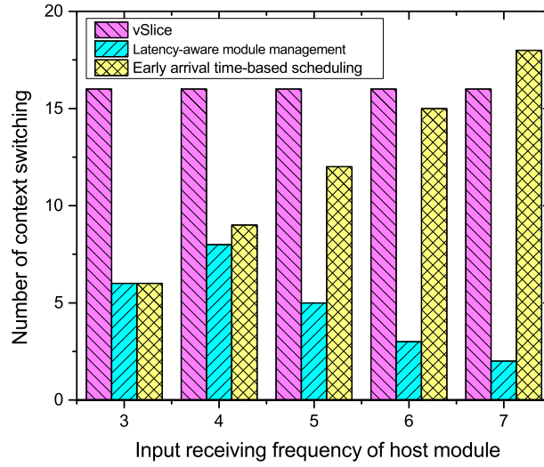
Figure 4.9: Number of context switches at different data receiving frequency of host
