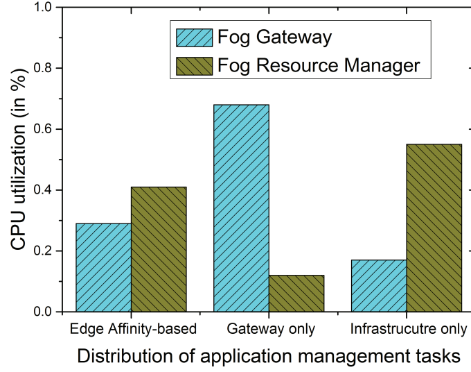
Figure 3.7: Average management load in different management setup
