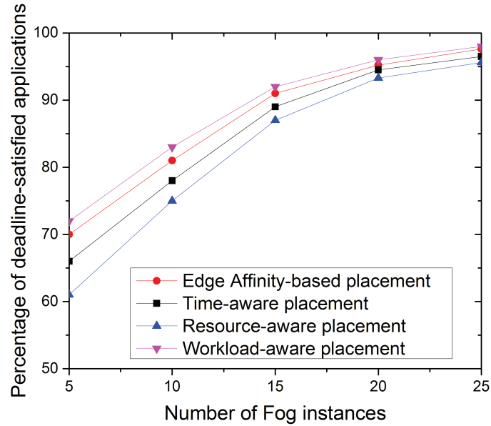
Figure 3.11: Percentage of QoS satisfaction for varying number of Fog instances
