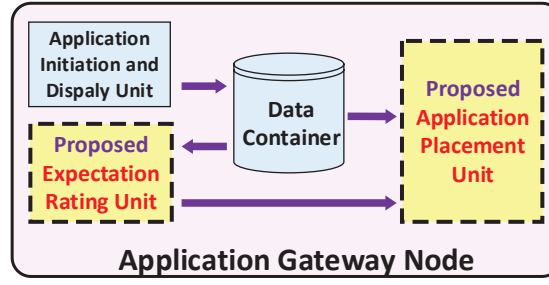
Figure 6.3: Architecture of a Fog gateway node
