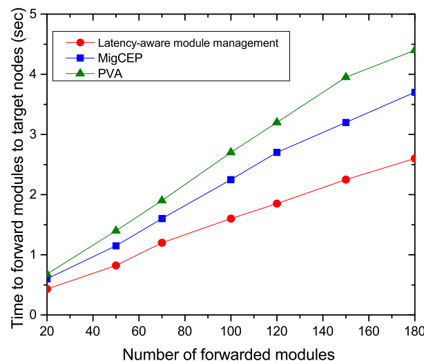
Figure 4.8: Required time for module forwarding
