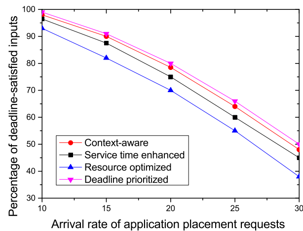
Figure 5.11: Percentage of deadline satisfaction for varying request arrival rate
