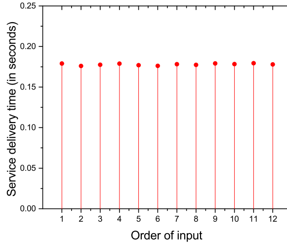
Figure 5.10: Service delivery time for different inputs of a stream
