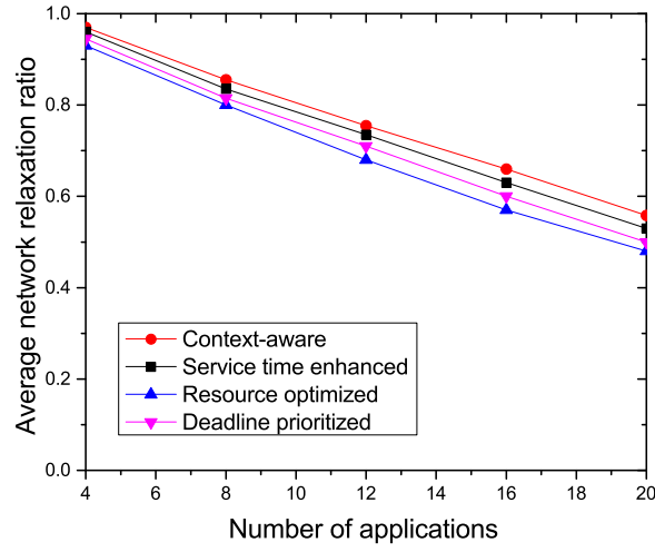
Figure 5.6: Average network relaxation for varying number of applications
