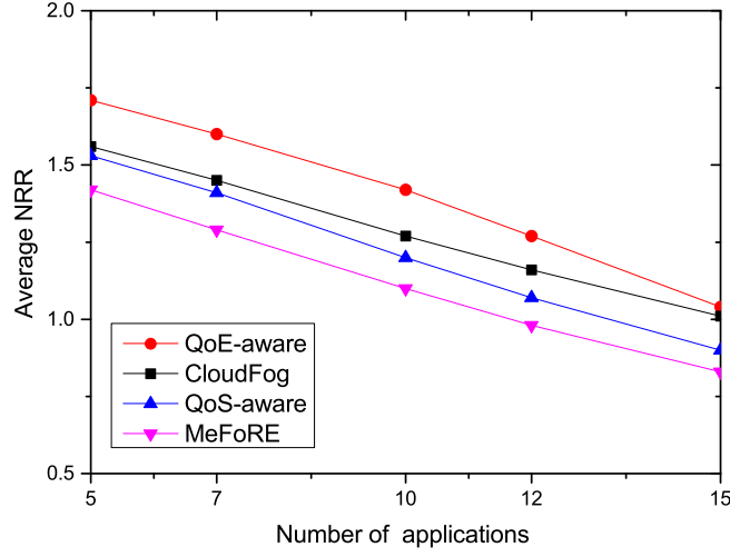
Figure 6.10: Network relaxation for varying number of applications
