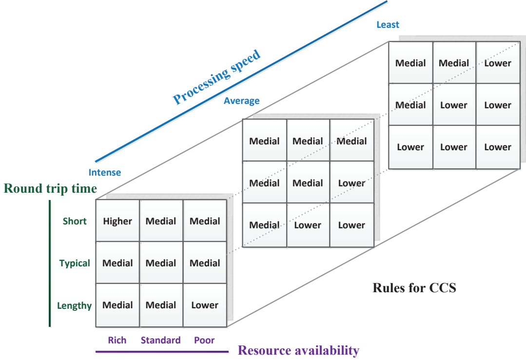
Figure 6.8: Fuzzy rules for CCS calculation
