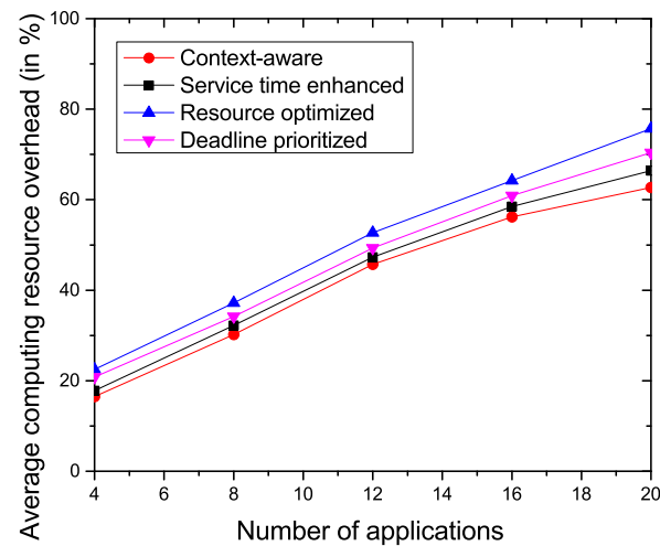
Figure 5.5: Average resource overhead for varying number of applications
