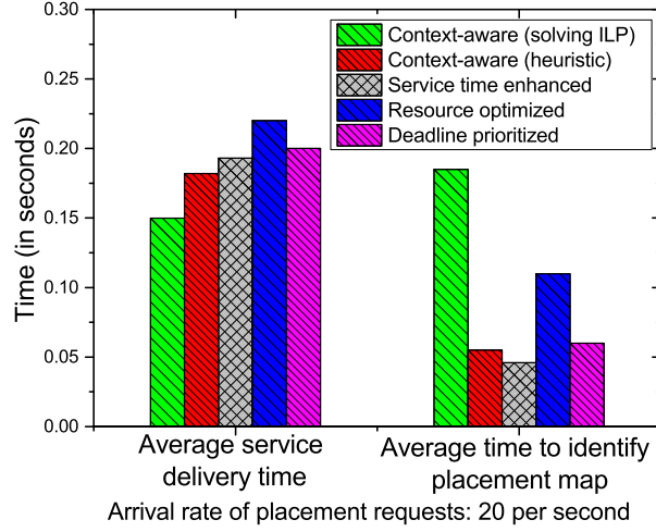
Figure 5.12: Average service and placement time for different placement policies
