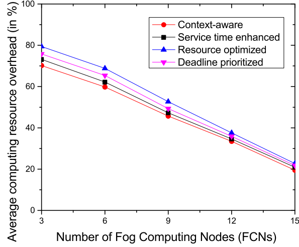
Figure 5.8: Average resource overhead for varying number of Fog nodes
