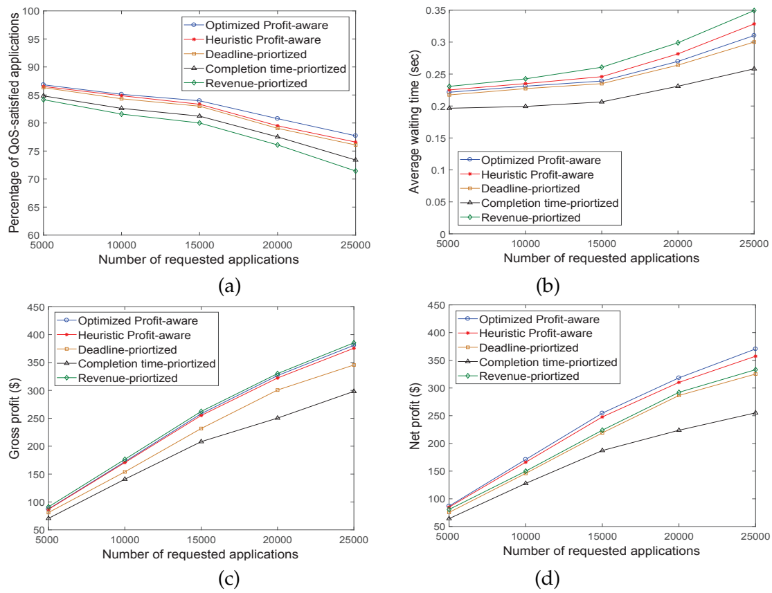
Figure 7.3: Impact of varying number of applications on (a) percentage of QoS satisfaction (b) waiting time (c) Gross profit (d) Net Profit
