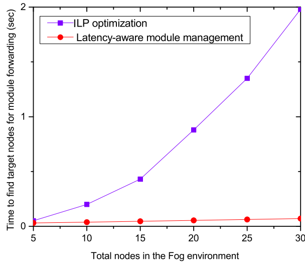
Figure 4.7: Required time for generating ILP and heuristic solutions
