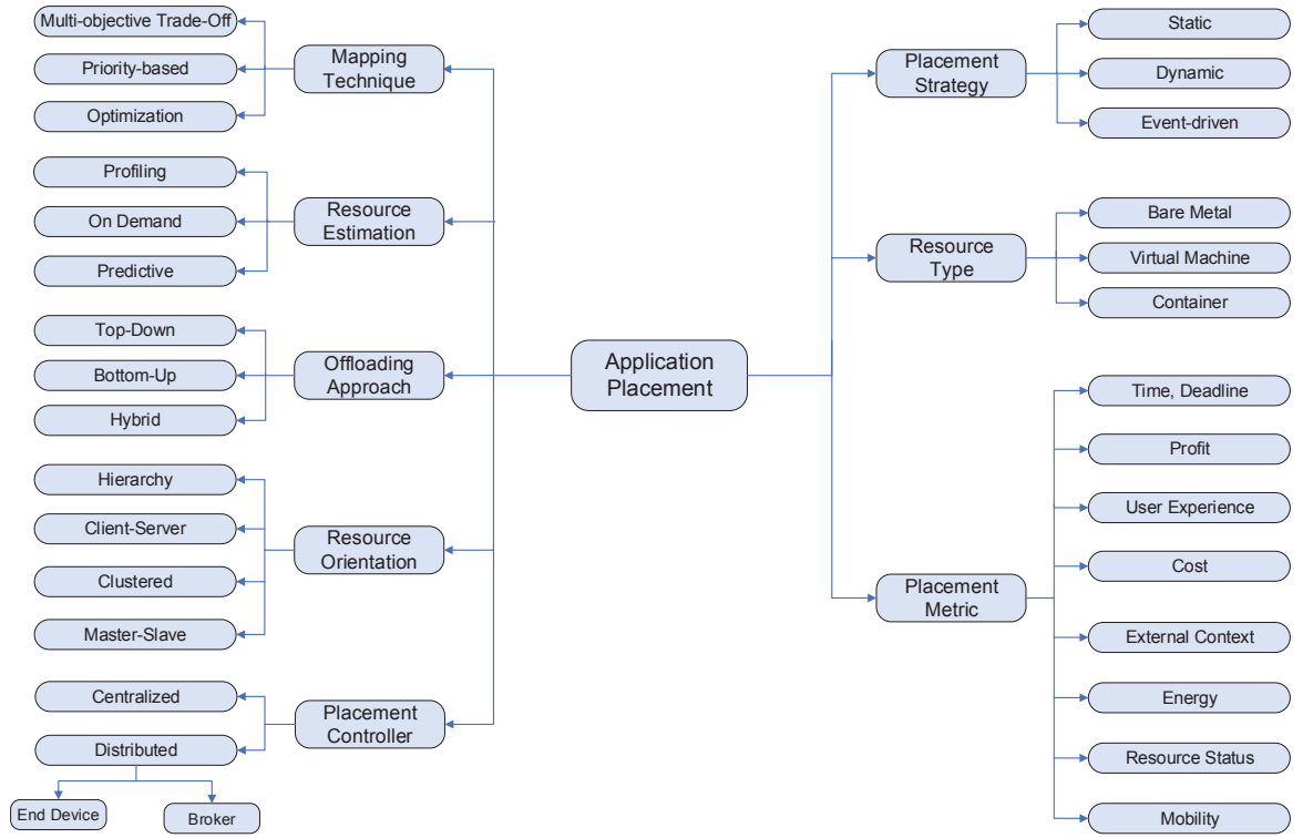
Figure 2.5: Taxonomy on application placement
