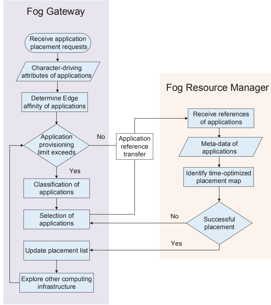
Figure 3.3: Flowchart for proposed Edge affinity-based application management
