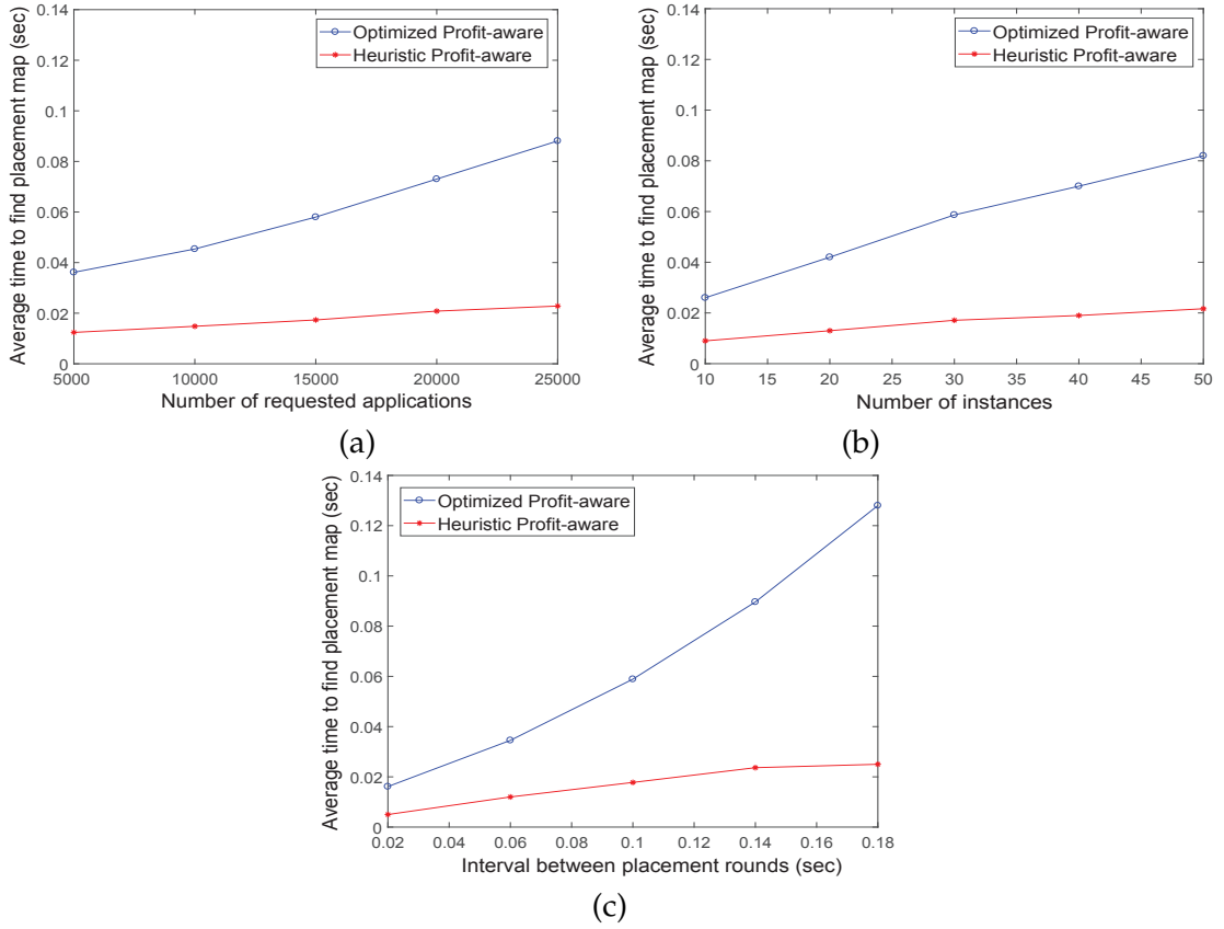
Figure 7.6: Required time to find placement map varying (a) number of requests (b) number of instances (c) placement round interval
