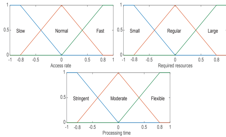
Figure 6.5: Membership function for expectation metrics
