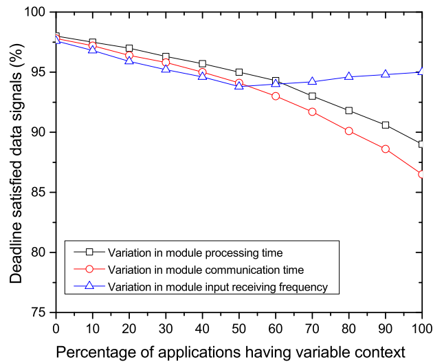
Figure 4.10: Performance of the proposed policy for varying application context
