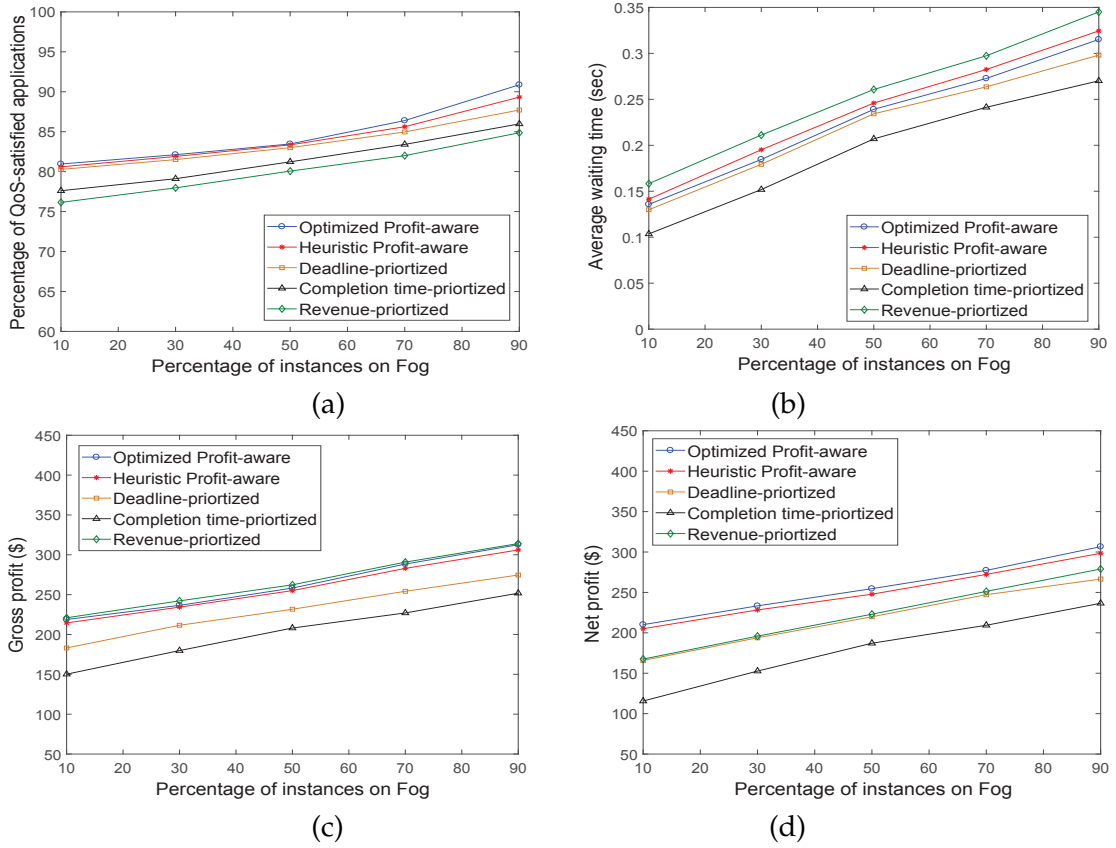
Figure 7.4: Impact of varying percentage of Fog instances on (a) percentage of QoS satisfaction (b) waiting time (c) Gross profit (d) Net profit
