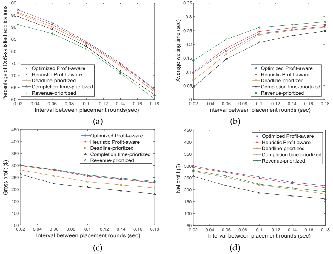
Figure 7.5: Impact of varying placement round interval on (a) percentage of QoS satisfaction (b) waiting time (c) Gross profit (d) Net Profit
