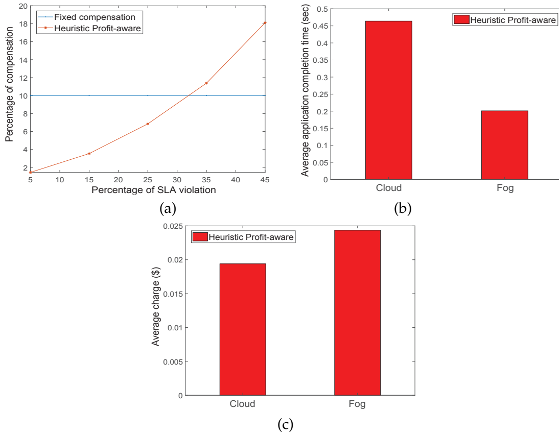
Figure 7.7: Comparison between (a) fixed and variable compensation (b) average application completion time (c) average charge for Fog and Cloud instances
