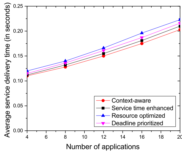
Figure 5.4: Average service delivery time for varying number of applications
