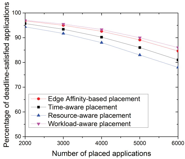
Figure 3.8: Percentage of QoS satisfaction for varying number of placed applications
