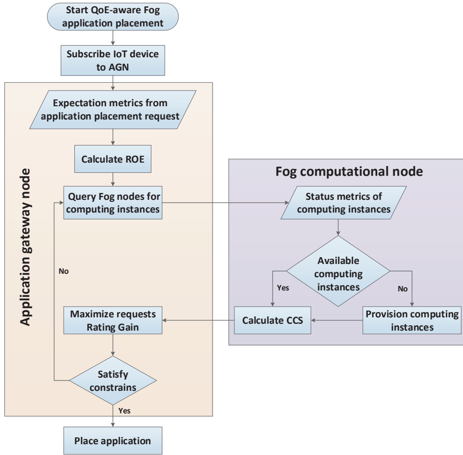
Figure 6.4: Flowchart for QoE-aware management
