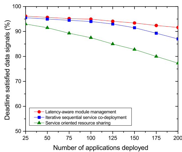
Figure 4.5: Percentage of QoS satisfaction for varying number of applications
