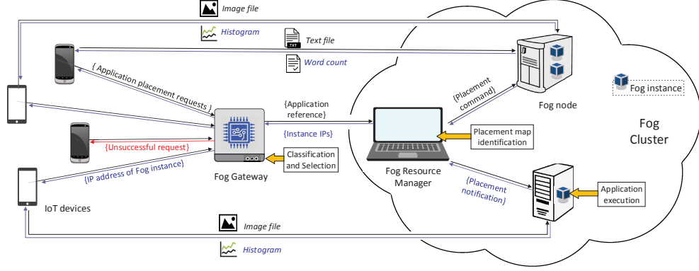
Figure 3.4: Real experimental setup for Edge affinity-based application management
