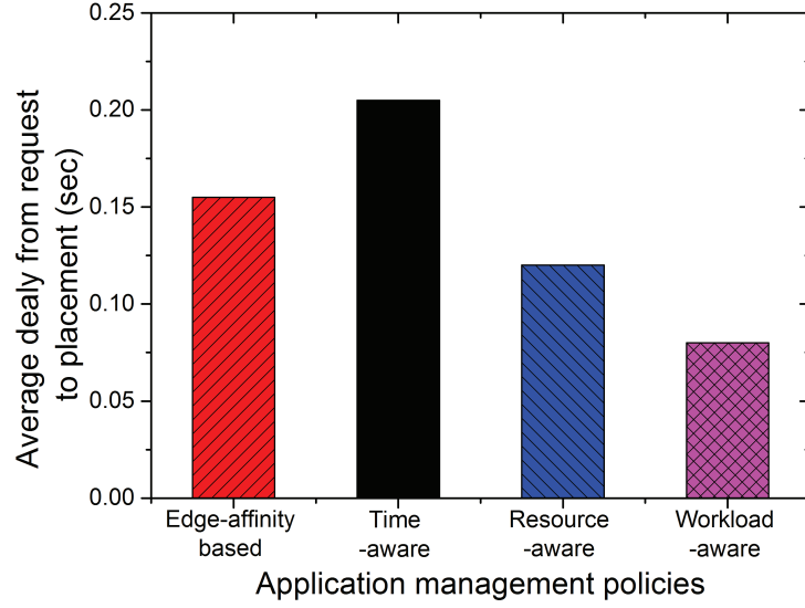
Figure 3.5: Average delay from request to placement for different management policies
