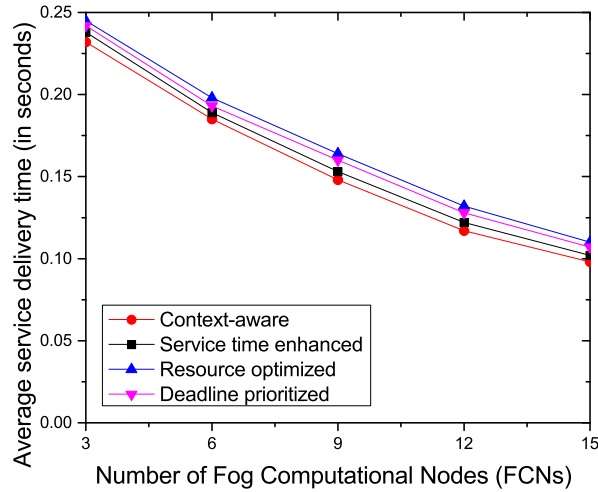
Figure 5.7: Average service delivery time for varying number of Fog nodes
