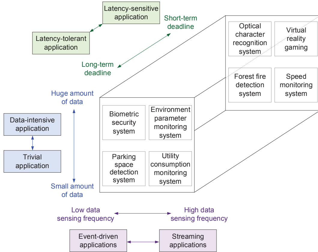
Figure 3.2: Variations of IoT applications
