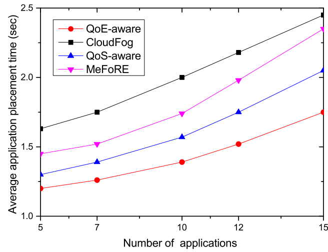
Figure 6.13: Application placement time for varying number of applications
