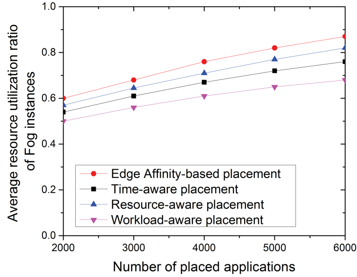
Figure 3.10: Average resource utilization for varying number of placed applications
