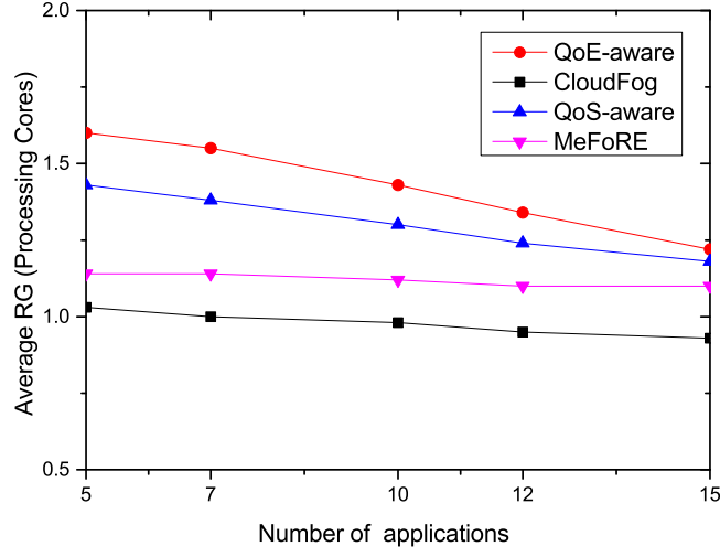
Figure 6.11: Resource gain for varying number of applications
