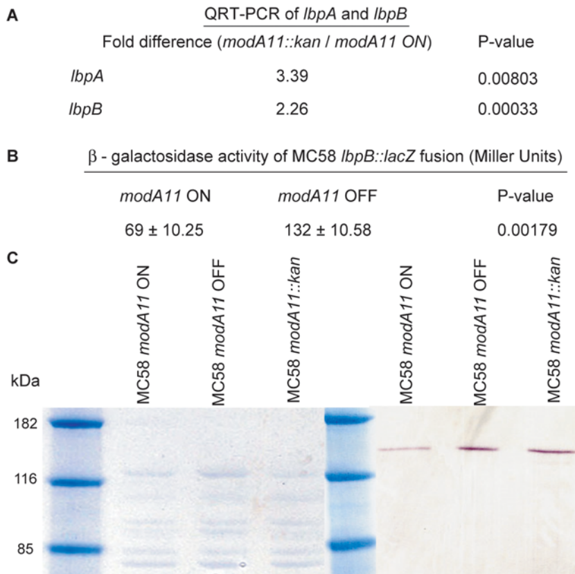
Figure 4. Analysis of wild-type MC58 modA11 ON, MC58 modA11 OFF, and MC58 modA11::kan for LbpA and LbpB expression. (A) Quantitative RT-PCR of lbpA and lbpB expression. Relative gene expression of lbpA and lbpB is higher in the MC58 modA11::kan mutant compared to wild-type MC58 modA11 ON. (B) Effect of modA11 phase variation on expression of the lbpB gene. \beta -galactosidase assays showed a statistically significant difference in the level of lbpB::lacZ gene expression resulting from modA11 repeat tract changes. A 1.9-fold difference in expression was observed between modA11 ON and modA11 OFF. P-values were calculated using a Student's t -test (C). The LbpA specific monoclonal antibody 296-H1 was used to assess expression of LbpA. The positions of molecular weight standard proteins are shown on the right in kilo Daltons (kDa). The left panel shows coomassie-stained wild-type MC58 modA11 ON, phase-variant MC58 modA11 OFF, and MC58 modA11::kan whole cells to show equal loadings of cell extracts. The right panel shows the Western blot of wild-type MC58 modA11 ON, phase-variant MC58 modA11 OFF, and MC58 modA11::kan whole cells probed with a monoclonal LbpA specific antibody. doi:10.1371/journal.ppat.1000400.g004
