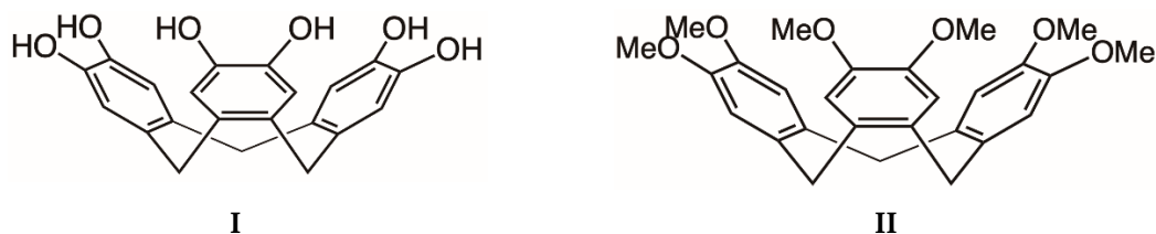
Scheme 1. Cyclotricatechylene ( I ) and cyclotrimeratrylene ( II ).
