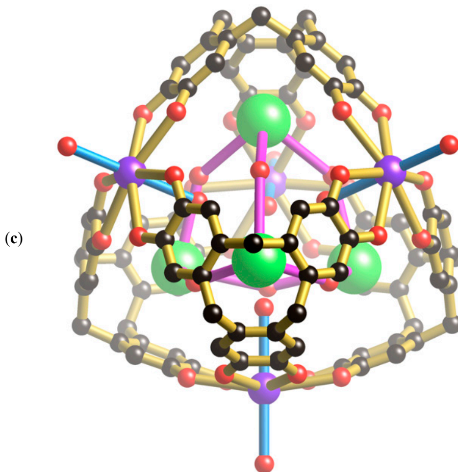
Figure 2. The structure of III showing (a) the [K_4(H_6ctc)_4(H_2O)_8]^{4+} cage (b) the [K_4(H_6ctc)_4(H_2O)_8]^{4+} cage indicating the topological relationship with a cube; each blue sphere represents a point on the 3-fold axis that passes through each of the H_6ctc molecules and (c) the [K_4(H_6ctc)_4(H_2O)_8]^{4+} cage showing the inclusion of the four internal Cs^+ ions and six water molecules; C black, O red, K purple, Cs green.
