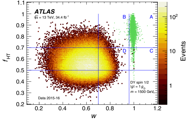
FIG. 1. Two-dimensional distribution of the two discriminating variables f_{\text{HT}} vs w in data (color scale) and a typical HIP signal (green squares). The regions for defining the signal (A) and for the background estimate and background validation (B, D, and C) are indicated.
