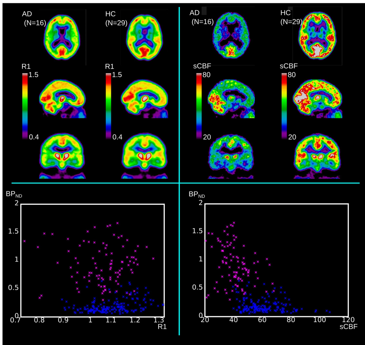
FIGURE 4 | Upper panels show mean values of R_1 and sCBF for comparison of AD to HC groups. Lower panels illustrate how relative R_1 and absolute sCBF measures differ in relation to BP_{ND} measures. Blue dots represent HC regional values (unilateral values of FL, PL, TL, and OL) and magenta dots represent similar regional values for AD subjects.
