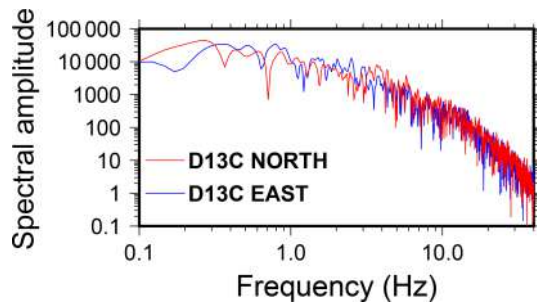
Figure 13. Velocity spectra for the 13 June 2011 M_w = 6 earthquake recorded at station D13C. No path corrections are applied.
