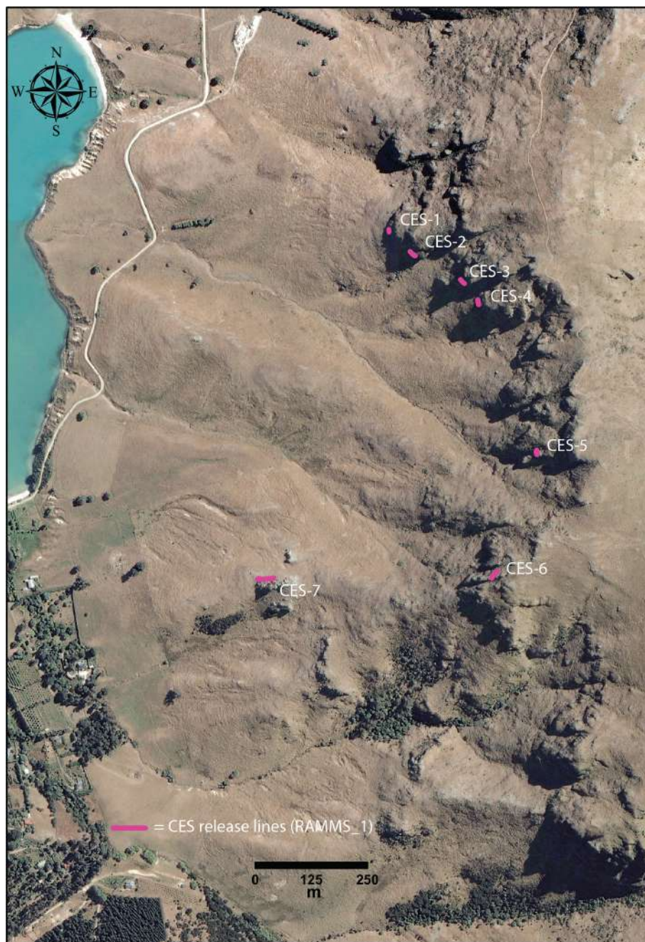
Figure A5. Polyline shapefiles for RAMMS_1 rockfall source areas. (Image is modified after Land Information New Zealand, https://data.linz.govt.nz/data/category/aerial-photos , last access: 6 March 2019.)
