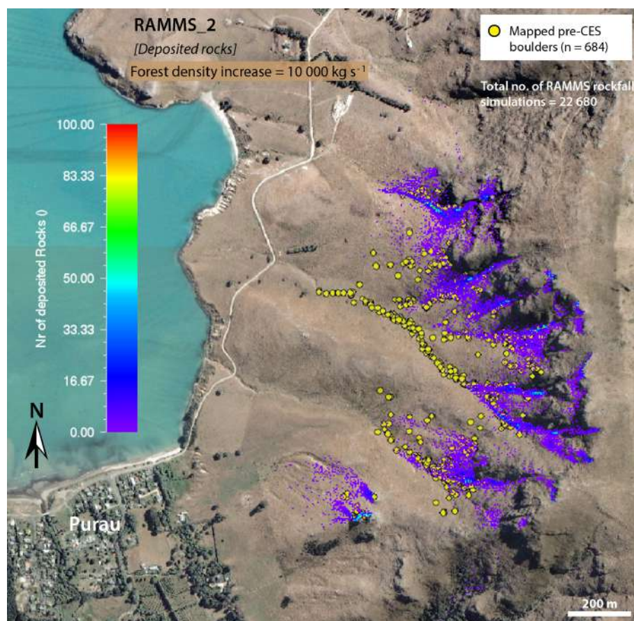
Figure A3. Final resting locations for RAMMS_2 rockfalls assuming uniform forest density increase of 10\,000\text{ kg s}^{-1} . (Image is modified after Land Information New Zealand, https://data.linz.govt.nz/data/category/aerial-photos , last access: 6 March 2019.)
