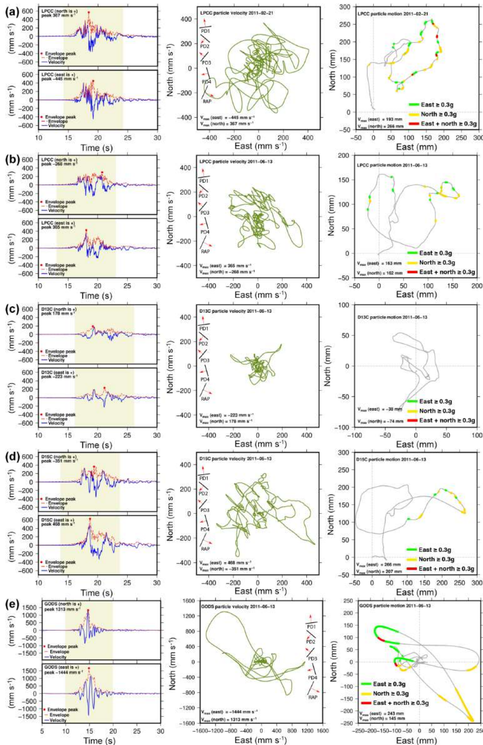
Figure 7. Each panel shows seismic data from LPCC (a, b), D13C (c), D15C (d), and GODS (e) stations. (a) and (b) compare ground motion, respectively, for 22 February 2011 M_w = 6.2 and 13 June 2011 M_w = 6 earthquakes at LPCC station. The left column shows east and north components of the velocity seismogram (blue line) and their respective envelopes (red dashed line). The particle velocity hodogram (middle column, green line) was determined for a time window \pm 5 s (shaded region in the left column) around the peak (red circle) of the east component envelope. The strike of the rock face (black short line segments) and the direction of the free face (red arrows) for sites PD1–PD4 and RAP are also illustrated. The particle motion hodogram (gray line) is presented in the right column, where green, yellow, and red segments represent, respectively, time points at which the east component, the north component, or both components exceed an acceleration of 0.3 g. Note that scale of figure axes varies by station particularly for ground motion.
