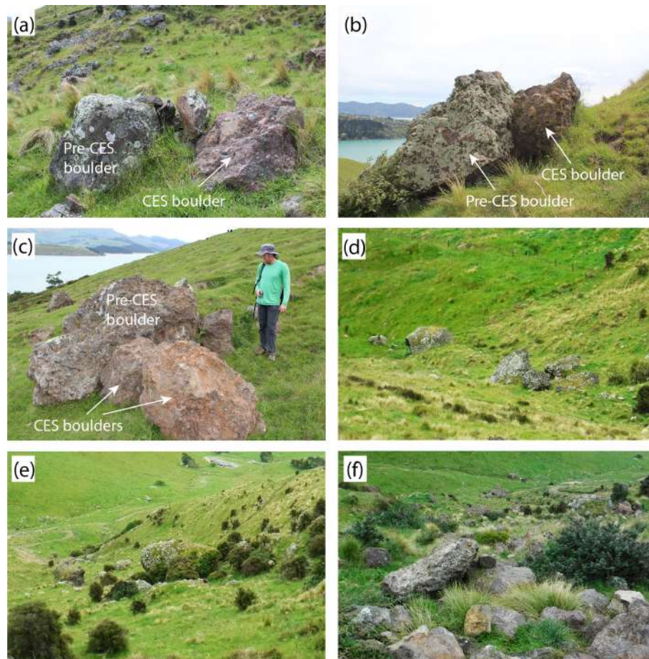
Figure 12. CES and pre-CES rockfall boulders within drainage valleys at Rapaki (a, c) and Purau (b, d–f) study locations. Drainage valleys contain a high amount of pre-CES rockfall boulders, which impacts the trajectory or path of CES rockfalls and reduces or stops runoff distance.
