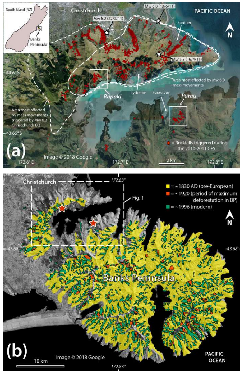
Figure 1. (a) © Google Earth image showing Rapaki and Purau study sites. CES rockfall locations as mapped by GNS Science and the authors (at Rapaki and Purau) are shown (red). Epicenter locations for 22 February, 13 June, and 16 April 2011 events are displayed (modified from Massey et al., 2014). Inset map of South Island (New Zealand) shows the Banks Peninsula and the approximate location for study site (yellow star). (b) Anthropogenic deforestation of Banks Peninsula (modified from Harding, 2003, and Wilson, 2013). Removal of native forest occurred rapidly in Banks Peninsula (BP) with the arrival of the Polynesians (1280 CE) then the Europeans (1830 CE). Before the Polynesian (Maori) arrival, extensive native forest was present throughout the BP. Prior to European settlement, minor to moderate removal of indigenous forest by Maori occurred, with burning being the primary tool for clearance (yellow). By 1920, Europeans had removed > 98 % of the BP native forest (red). Minor re-establishment of old-growth native forest has occurred (green), but slopes in the Port Hills and greater BP (including Rapaki and Purau) remain largely unvegetated.
