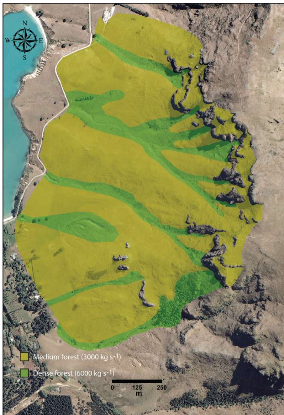
Figure A7. Polygon shapefiles for forest density. (Image is modified after Land Information New Zealand, https://data.linz.govt.nz/data/category/aerial-photos , last access: 6 March 2019.)
