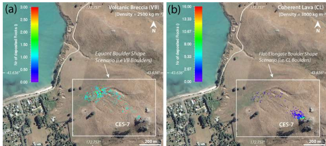
Figure 11. RAMMS simulated rockfall boulders showing differences in spatial distribution between VB (mostly equant shaped) and CL (predominantly elongate and flat shaped) boulder morphologies at Purau. All simulated boulders assume a volume of 1.0 \text{ m}^3 . (a) Spatial distribution of simulated VB boulders at Purau CES-7 location. Note the high relative percentage of simulated boulders deposited at the base of the hillslope ( \sim 500\text{--}600 \text{ m} from source rock). (b) Spatial distribution of simulated CL boulders at CES-7 location. Note the higher relative percentage of rockfall boulders deposited near the source rock (within \sim 100 \text{ m} from source rock). The simulation highlights the strong influence of boulder shape on runout distance. (All images are modified after Land Information New Zealand, https://data.linz.govt.nz/data/category/aerial-photos , last access: 6 March 2019.)
