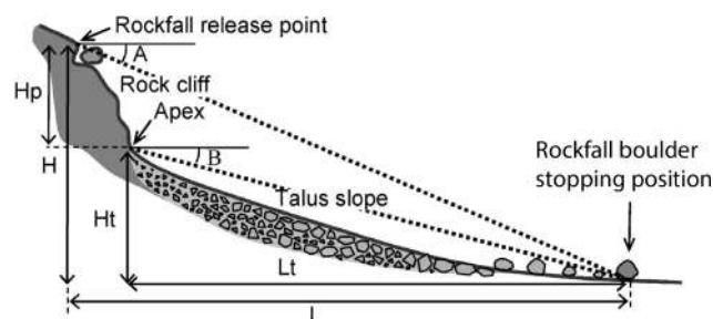
Figure A2. Conceptual diagram of hillslope illustrating the source rock cliff and the talus slope. The reach angle (a) and shadow angle (b) are shown. Sketch modified from Evans and Hungr (1993), Wieczorek et al. (2008), and Copons et al. (2009).
