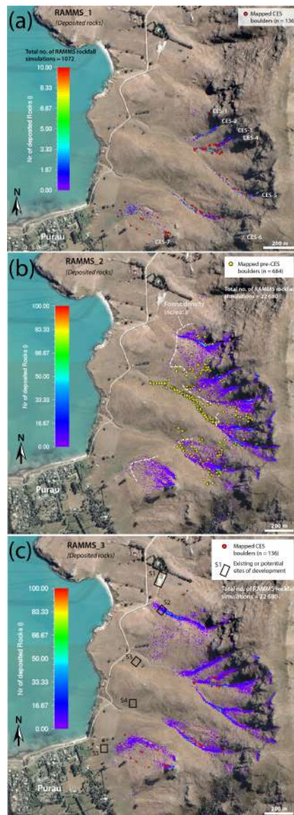
Figure 10. (a) RAMMS_1 shows deposited rocks for simulated CES boulders. Mapped CES boulders (red circles) are shown for comparison. Boulder densities of 2500 and 3000 kg m -3 are used for VB and CL boulders, respectively. (b) Final resting locations for RAMMS_2 rockfalls. RAMMS_2 assumes prehistoric rockfall conditions (i.e., forested hillslope). Mapped prehistoric rockfalls are depicted (yellow circles) for comparison. An increase in forest density to 10 000 kg s -1 generates the best fit with maximum runout distance (see white dashed line) for mapped prehistoric boulders. (c) Final resting locations for RAMMS_3 boulders. RAMMS_3 assumes modern hillslope conditions (i.e., deforested hillslope). Note the increased maximum runout distance for RAMMS_3 boulders compared with RAMMS_2 and the potential future rockfall hazard to development sites S1 and S2. The provided development sites are modified from Eliot Sinclair and Partners Ltd. (2013). (All images are modified after Land Information New Zealand, https://data.linz.govt.nz/data/category/aerial-photos , last access: 6 March 2019.)
