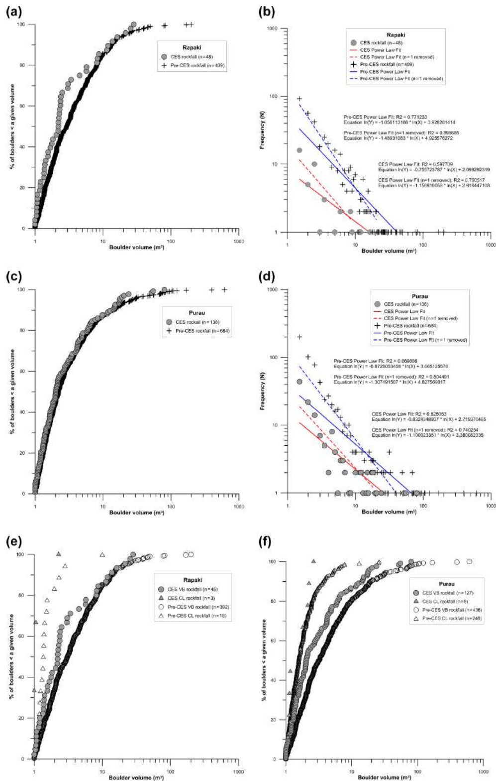
Figure 8. (a) Rockfall size distribution as a proportion of boulders less than a given size plotted in log space for CES and pre-CES rockfalls at Rapaki. (b) Rockfall frequency and size distribution for CES and pre-CES rockfalls at Rapaki. (c) Rockfall size distribution as a proportion of boulders less than a given size plotted in log space for CES and pre-CES rockfalls at Purau. (d) Rockfall frequency and size distribution for CES and pre-CES rockfalls at Purau. (e) Comparison of boulder size distributions for CES and pre-CES VB and CL rockfalls at Rapaki study site. (f) Comparison of boulder size distributions for CES and pre-CES VB and CL rockfalls at Purau.
