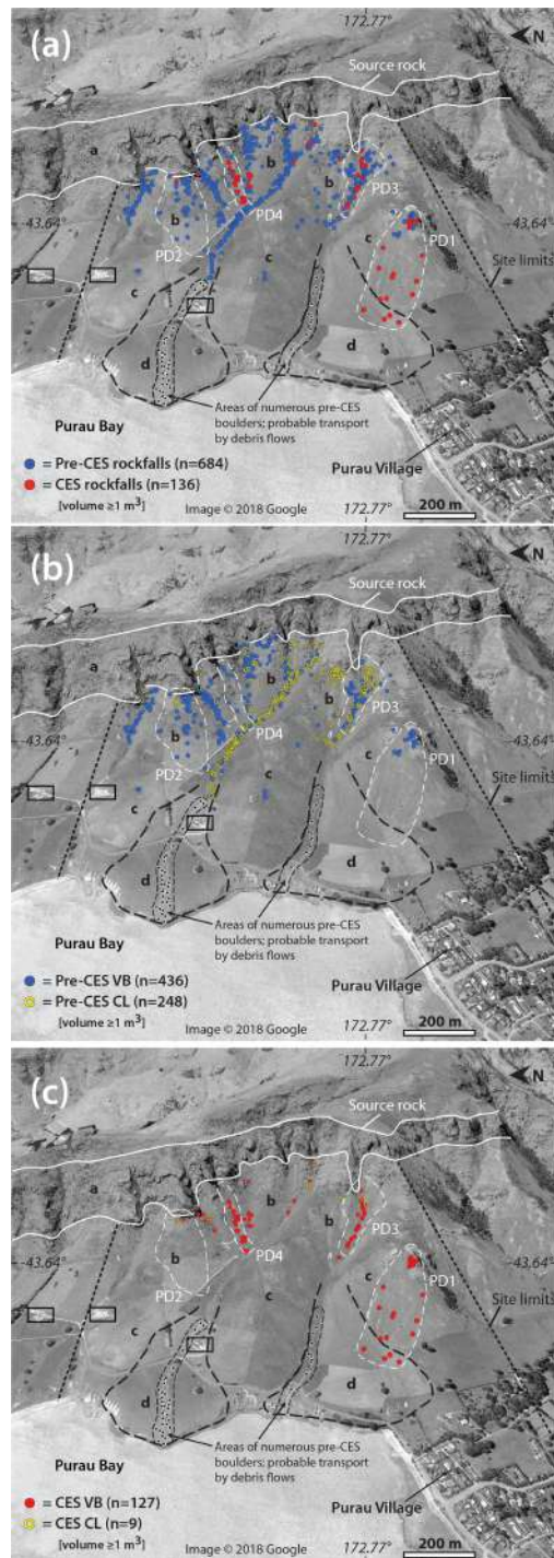
Figure 3. (a) Mapped pre-CES and CES rockfalls with volume \geq 1.0 \text{ m}^3 at Purau study site. Ratio of pre-CES to CES boulders is \sim 5 : 1 (a: volcanic source rock; b: dominated by volcanic boulder colluvium and volcanic loess colluvium; c: loess colluvium underlain by in situ loess and volcanic rock; d: alluvial sediments overlying loess and bedrock). (b) Mapped pre-CES VB and CL boulders at Purau. Ratio of pre-CES VB to CL boulders is \sim 2 : 1 . (c) Mapped CES VB and CL boulders at Purau study site. Note the low number of CL rockfall boulders detached during the CES at Purau. Ratio of CES VB to CL boulders is \sim 14 : 1 . PD1–PD4 represent Purau rockfall domains.
