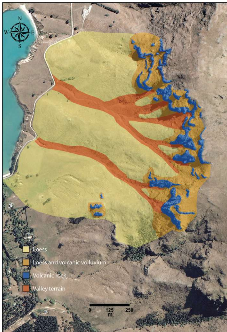
Figure A4. Polygon shapefiles for runout terrain types. (Image is modified after Land Information New Zealand, https://data.linz.govt.nz/data/category/aerial-photos , last access: 6 March 2019.)
