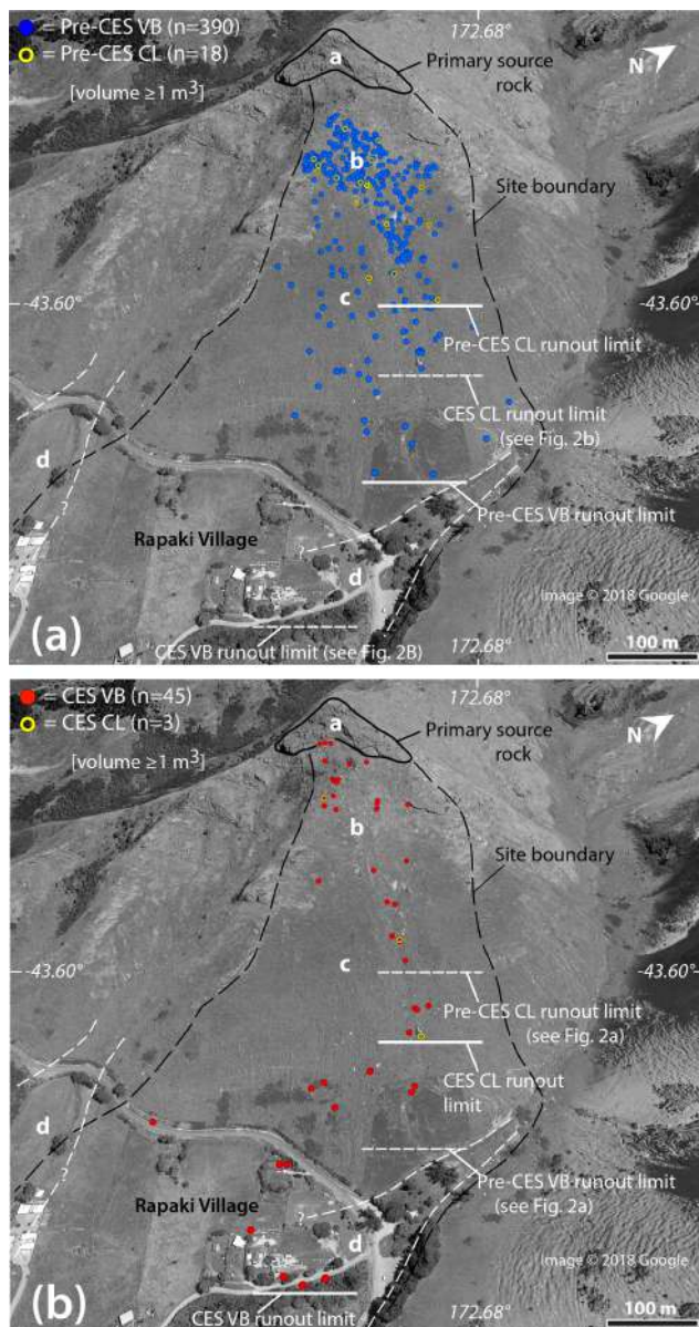
Figure 2. (a) Mapped pre-CES volcanic breccia (VB) and coherent lava (CL) boulders with volume \geq 1.0 \text{ m}^3 at Rapaki. The largest boulders with the furthest runout distances are comprised exclusively of volcanic breccia. Ratio of pre-CES VB to CL boulders is \sim 22 : 1 . (b) Mapped CES VB and CL boulders at Rapaki study site. Note the low number of CL rockfall boulders detached during the CES at Rapaki. Ratio of CES VB to CL boulders is 15 : 1 (a: volcanic source rock; b: dominated by volcanic boulder colluvium and volcanic loess colluvium; c: loess colluvium underlain by in situ loess and volcanic rock; d: alluvial sediments overlying loess and bedrock).
