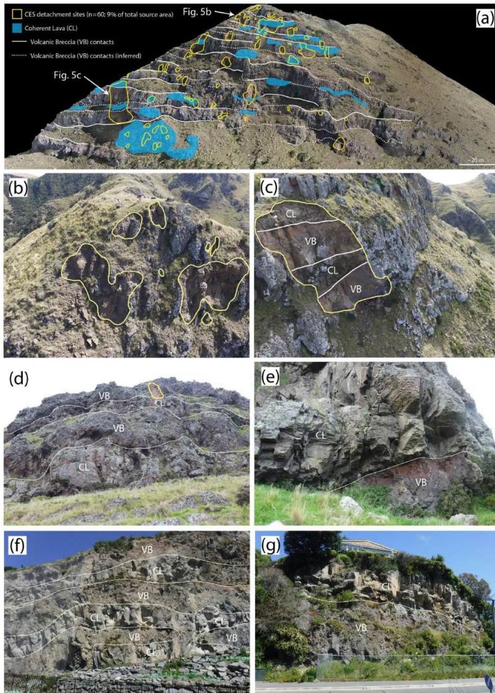
Figure 5. (a) Volcanic source rock at Rapaki study site. Sixty individual detachment zones were created during the CES (yellow) and represent \sim 9\% of the total source rock area. The source rock is comprised of \sim 86\% VB and \sim 14\% CL. Approximately \sim 69\% and \sim 31\% of the detachments occurred within the VB and CL lithologies, respectively. (b) Photo showing several irregularly shaped CES detachment zones near the top of Mount Rapaki. (c) Photo showing freshly exposed VB and CL layering within the Rapaki source rock. (d) Portion of volcanic source rock at Purau showing VB and CL layering. A single CES detachment site is shown at the top of the source rock. Seven individual CES detachment sites were identified at the Purau study site. (e) CL and VB layers at the Purau study site. Note the thickness of the CL layer ( \sim 5\text{--}7\text{ m} ) and lack of any CES detachment sites despite the high degree of fracturing and overhanging condition. (f) VB and CL layering in Sumner (Christchurch) cliff exposure adjacent to Main Road. Extensive cliff collapse during the CES has revealed multiple lava flows and the distinctive textural differences between the VB and CL lithologies. Note the high density of vertical to subvertical fractures within the CL layers. (g) Exposed lava layers adjacent to Main Road in Redcliffs (Christchurch). Note the single-family living residence at top of photo.
