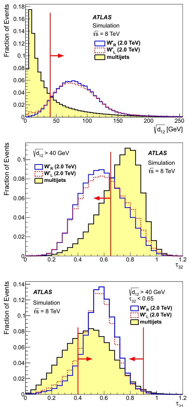
Fig. 1 Distributions in simulated samples of the substructure observables used for the W' top-tagger for trimmed large- R jets originating from QCD-multijet production and originating from hadronic decays of top quarks from 2 TeV W'_L and W'_R boson decays. The top figure shows the \sqrt{d_{12}} distributions and the middle ( bottom ) figures show the \tau_{32} ( \tau_{21} ) distribution after requiring \sqrt{d_{12}} > 40 GeV ( \sqrt{d_{12}} > 40 GeV and \tau_{32} < 0.65 ). All distributions are normalised to unity. The arrows indicate the cut values used in the W' top-tagger
