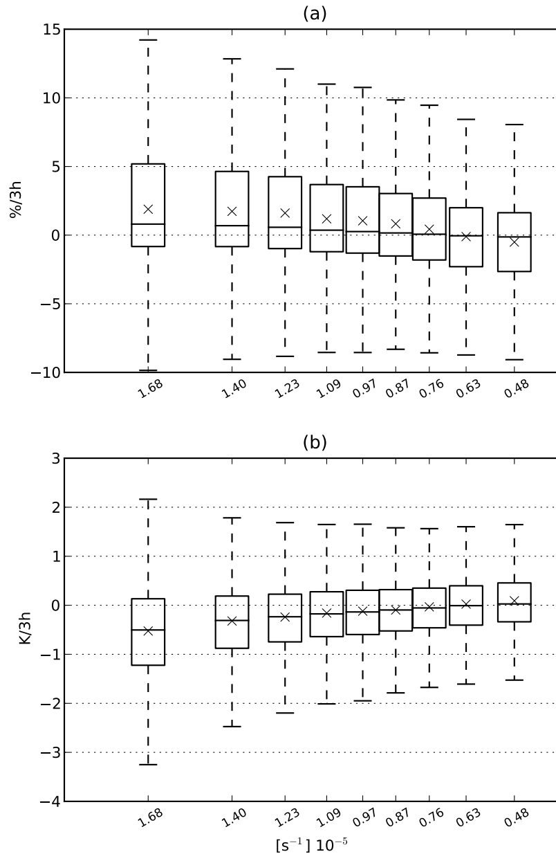
Figure 10. Temporal changes in (a) sea ice concentration and (b) surface temperature versus wind convergence (horizontal axis). Selected systems were generated south of 55°S and located over the partially ice covered ocean. Boxes present data divided by 10, 20, ..., 90% percentile values of wind convergence and extend from the lower to upper quartile values of the data, with a line at the median. Whiskers extend from 25% to 75% of data and means are marked with crosses.
