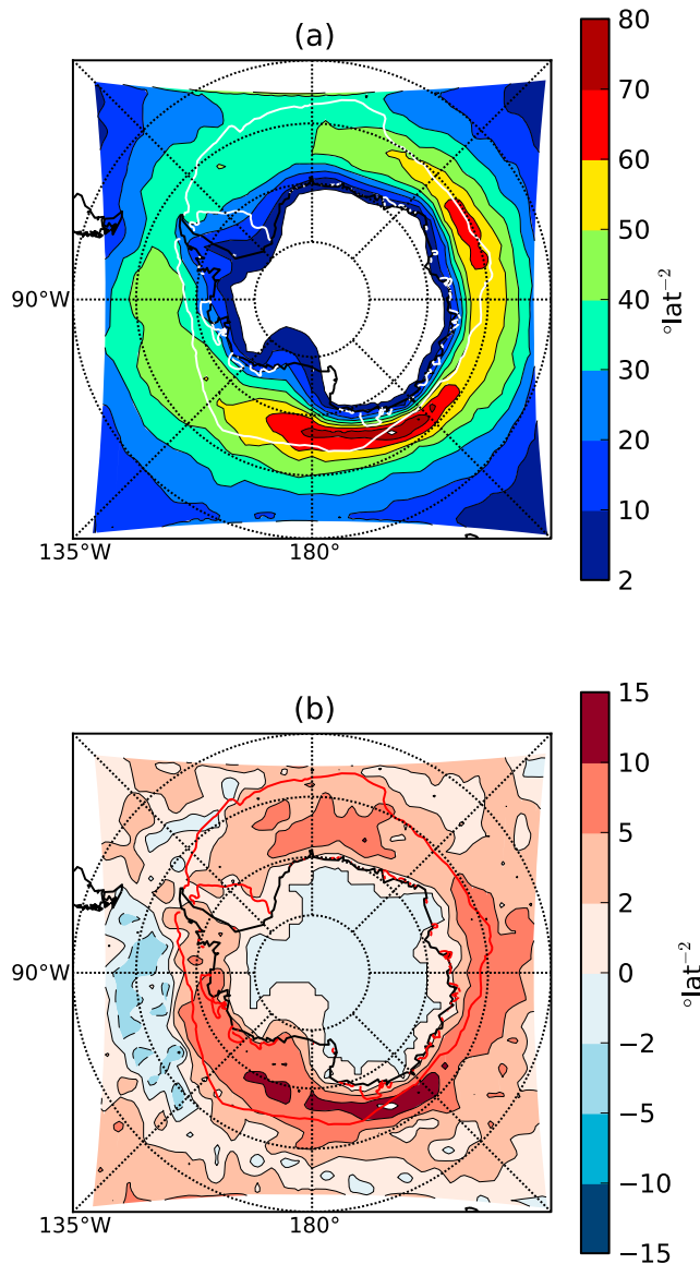
Figure 3. Track densities (the number of tracks per ^{\circ}\text{latitude}^2 ) of (a) cyclones with maximum radius larger than 4.5^{\circ}\text{latitude} and (b) their difference between winter and summer (JJA–DJF). Continuous lines mark the isolines of 70% mean ice concentration for 2001–2007 in February (inner line) and in September (outer line) around Antarctica.
