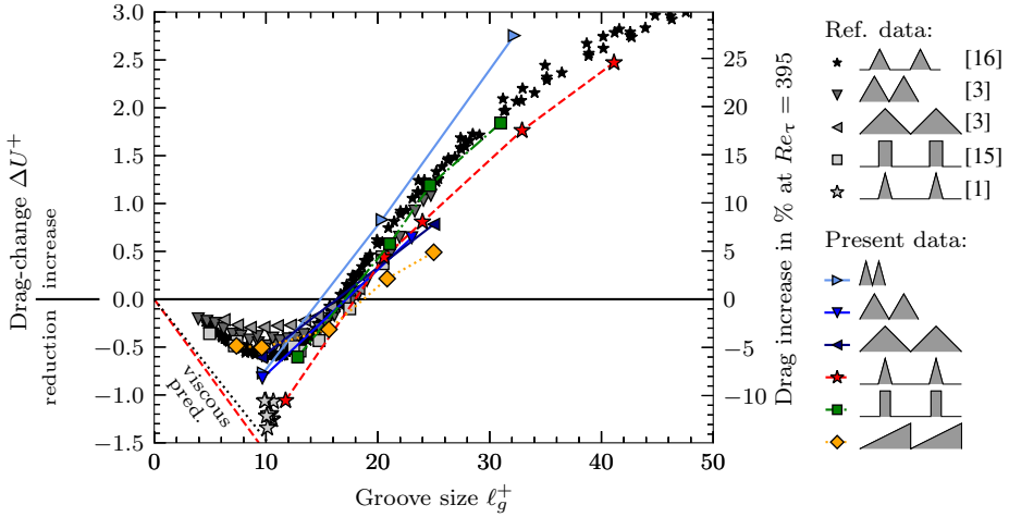
Fig. 9 Drag curves for different riblet shapes with experimental (★ [16], ▼ [3], ◄ [3]) and numerical (DNS: ◻ [15], LES: ☆ [1]) reference data. Experimental channel flow data are converted from \Delta\tau_w/\tau_{w,\text{smooth}} to \Delta U^+ = -\text{DR}((2c_{f,\text{smooth}})^{-1/2} + 1/(2\kappa)) with c_f = 2/U_{\text{bulk}}^{+2} at matched Re_{\text{bulk}} [3]. The term 1/(2\kappa) is omitted for data from [3] as suggested in [12]. The boundary layer LES data are converted to \Delta U^+ = -\text{DR}(2C_{f,\text{smooth}})^{-1/2} with C_f = 2/U_\delta^{+2} at matched U_\delta^+ [37]. Direct measurements of \Delta U^+ for the present data are shown by coloured symbols with lines. The straight lines starting at \ell_g^+ = 0 indicate the viscous prediction of \Delta U^+ calculated from Stokes flow as per [28], for trapezoidal riblets with \alpha = 53.5^\circ (⋯⋯, as [16]) and \alpha = 30^\circ (---, as [1] and our data).
