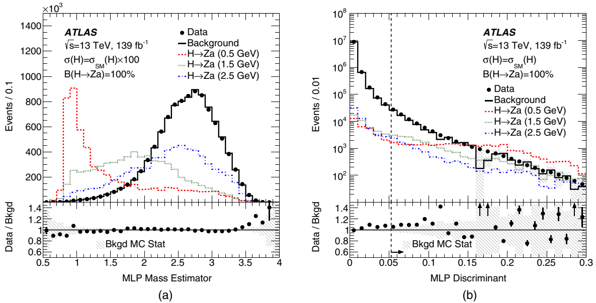
FIG. 1. Output of (a) the regression and (b) the classification MLPs, for data, background, and three signal hypotheses. Events are required to pass the complete event selection, including the 120 < m_{\ell\ell j} < 135 GeV requirement, but not the requirement on the classification MLP output variable. The background normalization is set equal to that of the data, and the signal normalizations assume the SM Higgs boson inclusive production cross section and \mathcal{B}(H \rightarrow Za) = 100\% , and in (a) the signal normalization is scaled up by a factor of 100. The error bars (hatched regions) represent the data (MC) sample statistical uncertainty, in both the histograms and the ratio plots. In (b) the region to the right of the dashed line is the signal region.
