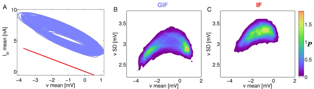
Figure 10. Mean and standard deviation of the membrane potential across neurons. A: Covariation of the mean membrane potential and the mean intrinsic current across neurons in the GIF (blue) and IF (red) networks. B, C: Bivariate probability density function of the mean and standard deviation of the membrane potential variable across neurons for the GIF (B) and IF (C) networks. Brighter colors indicate higher probabilities. doi:10.1371/journal.pcbi.1003574.g010
