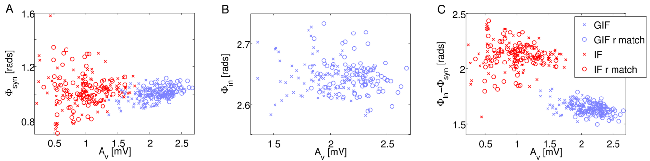
Figure 9. Phase relationships of synaptic and intrinsic currents and their effect on synchrony A: Phase of the sinusoidal fit to the mean synaptic current I_{\text{syn}} plotted against the local level of synchrony (as assessed by the amplitude of the sinusoidal fit to the mean membrane potential A_v ). GIF: blue; IF: red. Crosses: canonical models; circles: r-matched models. B: As in A, for the mean intrinsic current I_{\text{in}} . Only GIF networks are shown, as \Phi_{\text{in}} is always equal to \pi in IF networks. C: As in A, for \Phi_{\text{in}} - \Phi_{\text{syn}} . doi:10.1371/journal.pcbi.1003574.g009
