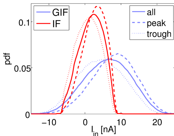
Figure 7. Distribution of intrinsic currents conditioned on the phase of the population rhythm. Probability density functions of intrinsic currents I_{in} in the GIF (blue) and IF (red) networks. Solid lines indicate unconditional probability densities, dashed (dotted) lines indicate probability densities conditioned on the peak (trough) of the mean I_{in} oscillation. doi:10.1371/journal.pcbi.1003574.g007
