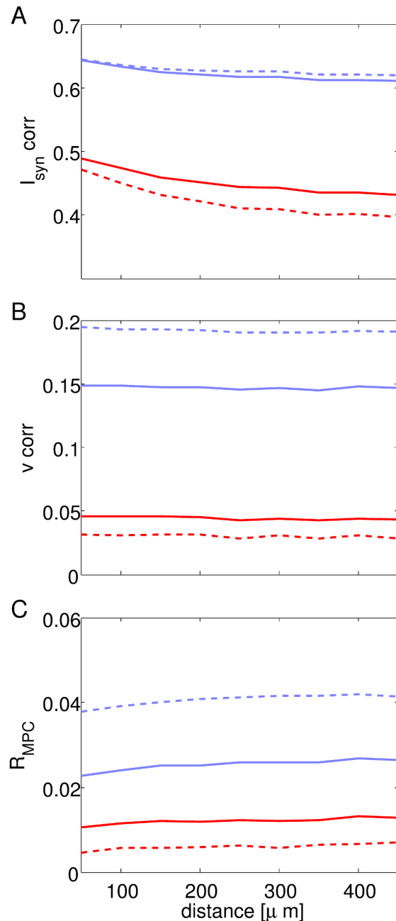
Figure 4. Correlation between synaptic inputs, membrane potential trajectories and R_{MPC} among pairs of neurons as a function of distance. A: Average Pearson correlation between incoming synaptic currents to neuron pairs as a function of their distance. Note the high correlation for nearby neurons, which decreases with distance. B: Average Pearson correlation between the membrane potential of neuron pairs as a function of their distance. The modulation with distance is negligible. C: R_{MPC} between firing patterns of neuron pairs as a function of their distance. R_{MPC} decreases at short distances due to short-latency mutual inhibition. Line styles and colors as in Figure 3. doi:10.1371/journal.pcbi.1003574.g004
