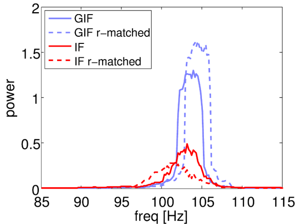
Figure 3. Power spectrum of population activity. Power spectrum of the population rate R_p for the four model networks considered. Population activity exhibits a peak at \sim 100 Hz, with higher synchrony corresponding with slightly higher population frequency. Note the tall, non-Gaussian peaks in the GIF networks, corresponding to non-linear, fully developed oscillations. In contrast, power spectrum peaks in the IF networks are bell-shaped, a signature of sinusoidal oscillations. doi:10.1371/journal.pcbi.1003574.g003
