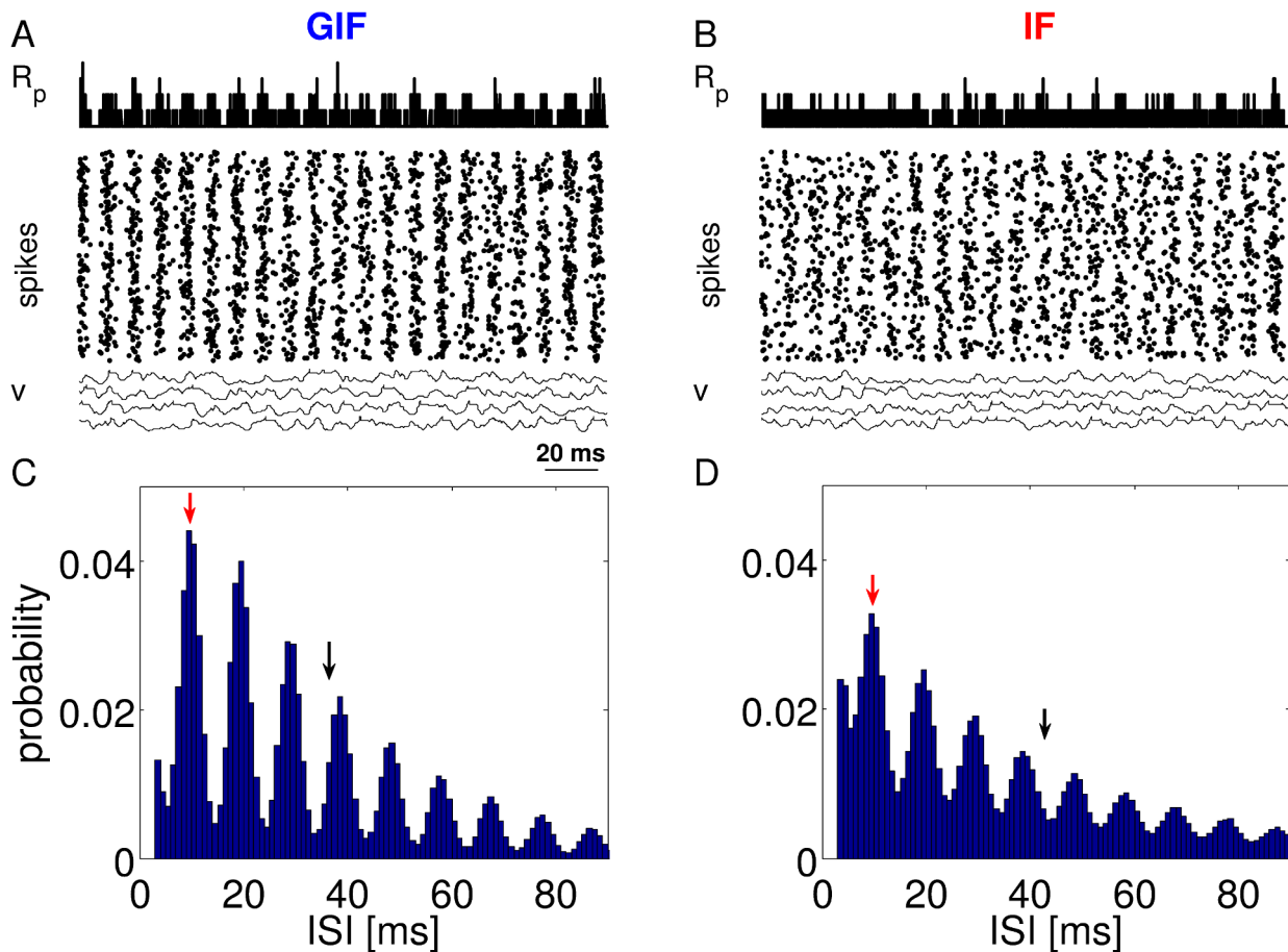
Figure 2. Sample activity in the canonical GIF and IF networks. A: Population rate (top), spike raster plot (middle), and v trajectories of selected neurons (bottom) in the GIF network for a representative parameter set. C: Single-cell ISI histogram for the GIF network. The red arrow indicates the period of network oscillations. The black arrow indicates the mean single-cell ISI. B, D: The same as A and C, for the IF network. Oscillations are more prominent in the GIF network. doi:10.1371/journal.pcbi.1003574.g002
