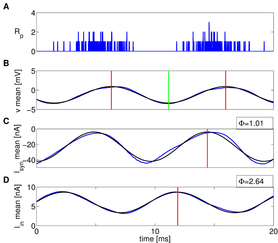
Figure 6. Intrinsic and synaptic currents. Population rate R_p (A), along with the mean membrane potential v (B), the mean synaptic current I_{syn} (C), and the mean intrinsic current I_{in} (D) across neurons for the GIF network in a short representative time window. Blue lines show simulation results, black lines are least-squares sinusoidal fits. The red vertical lines indicate the peak of the sinusoidal fit to the corresponding traces, the green vertical line indicates the trough of the sinusoidal fit to the mean membrane potential oscillation. Phase leads ( \Phi , in radians) with respect to the mean membrane potential oscillation are shown for the mean synaptic current I_{syn} and the mean intrinsic current I_{in} . doi:10.1371/journal.pcbi.1003574.g006
