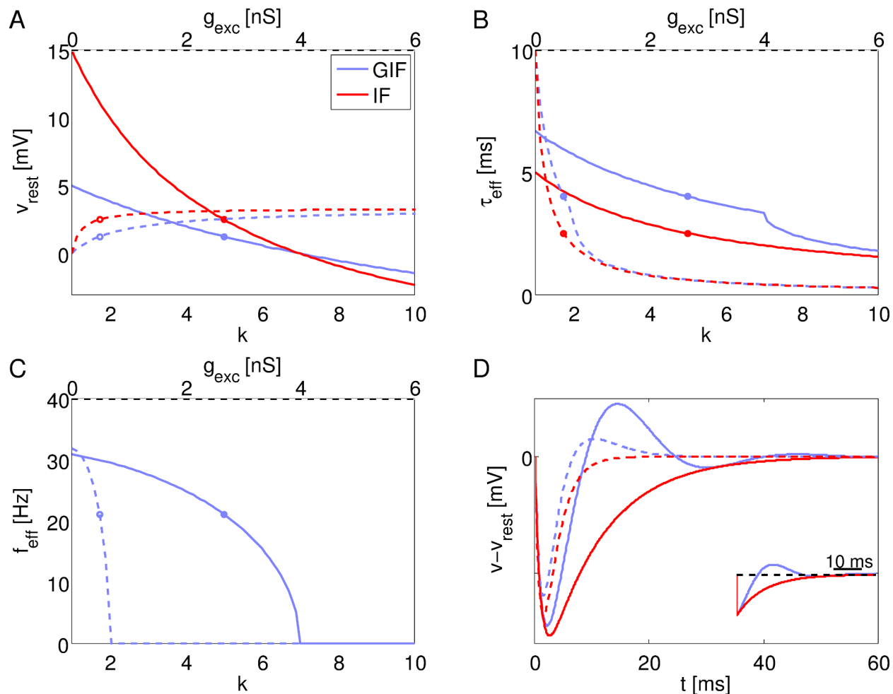
Figure 1. Linear analysis of the neuron models. Linear analysis of the model neurons with fixed external conductances. A: Resting potential as a function of the background inhibition-to-excitation ratio k for the canonical value of g_{\text{exc}} (solid lines), and as a function of the background synaptic excitation g_{\text{exc}} for the canonical value of k (dashed lines). Solid lines refer to the bottom axis; dashed lines to the top axis. Circles show the canonical values of the corresponding parameters. B: Effective membrane time constant as a function of k and g_{\text{exc}} . Line styles, colors and symbols as in A. C: Effective intrinsic frequency as a function of k and g_{\text{exc}} . Line styles, colors and symbols as in A. D: IPSPs in response to a single presynaptic pulse delivered at time t = 0 , in the presence (dashed lines) or absence (solid lines) of fixed background conductances. Inset shows the membrane potential response to an instantaneous perturbation. doi:10.1371/journal.pcbi.1003574.g001
