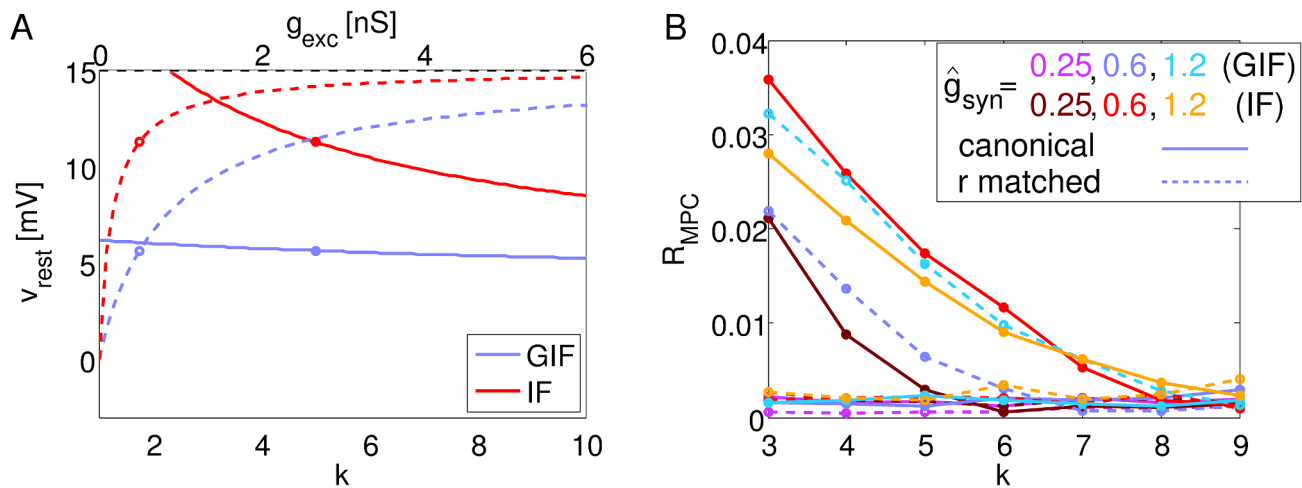
Figure 11. Neuronal dynamics if inhibition is shunting, rather than hyperpolarizing. A: Resting potential as a function of the background inhibition-to-excitation ratio k for the canonical value of g_{exc} (solid lines), and as a function of the background synaptic excitation g_{exc} for the canonical value of k (dashed lines). Solid lines refer to the bottom axis; dashed lines to the top axis. Circles show the canonical values of the corresponding parameters. All parameters as in Table 1, except E_{inh} = 4 mV. Compare with analogous results for hyperpolarizing inhibition shown in Figure 1A. B: Synchrony (as assessed by R_{MPC} ) as a function of the background inhibition-to-excitation ratio k for different values of the coupling strength \hat{g}_{syn} . Voltage threshold for spike generation v_{thr} has been increased to 15 mV in the canonical models, in order to compensate for the depolarization of the resting potential and to keep the models in the fluctuation-driven regime. Voltage thresholds for r -matched models have been scaled accordingly for each value of k . GIF: purple, weak coupling ( \hat{g}_{syn} = 0.25 \mu S); blue, medium coupling ( \hat{g}_{syn} = 0.6 \mu S); light blue, strong coupling ( \hat{g}_{syn} = 1.2 \mu S). IF: brown, weak coupling; red, medium coupling; orange, strong coupling. All other parameters as in Table 1, except E_{inh} = 4 mV, v_{reset} = 4 mV. Dots indicate simulated points, lines are drawn to guide the eye. doi:10.1371/journal.pcbi.1003574.g011
