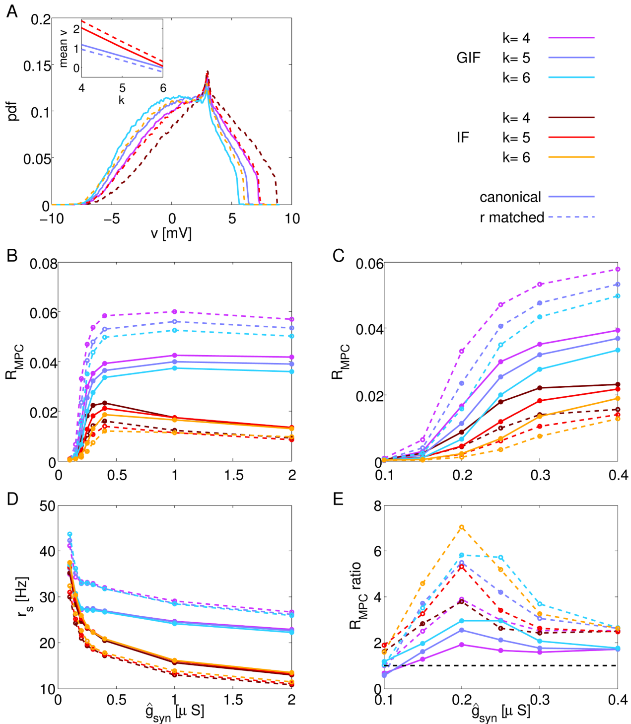
Figure 5. Effects of membrane potential depolarization and coupling on network dynamics. A: Membrane potential distributions of GIF and r-matched IF neurons in response to the background input alone, for different values of the background inhibition-to-excitation ratio k . In all cases, the voltage threshold for spike generation v_{thr} has been adjusted in order to match the rate response of the canonical GIF (73.7 Hz). Color and line style code as indicated. Inset shows the mean membrane potential as a function of k for the four model networks shown in Figure 3 (same line colors and styles). B, D: Synchrony (as assessed by R_{MPC} , B) and firing rates (D) as a function of coupling strength \hat{g}_{syn} . C: Enlarged view of B for low values of coupling strength. E: Ratio between corresponding curves in C. Solid lines show ratios between canonical models ( R_{MPC}(\text{GIF})/R_{MPC}(\text{IF}) ), while dashed lines show ratios between models that have been adjusted in order to exhibit the same rate response to the background input (purple, blue and light blue, R_{MPC}(\text{GIF})/R_{MPC}(\text{r-matched IF}) ; brown, red and orange, R_{MPC}(\text{r-matched GIF})/R_{MPC}(\text{IF}) ). Dots in B–E indicate simulated points, lines are drawn to guide the eye.
