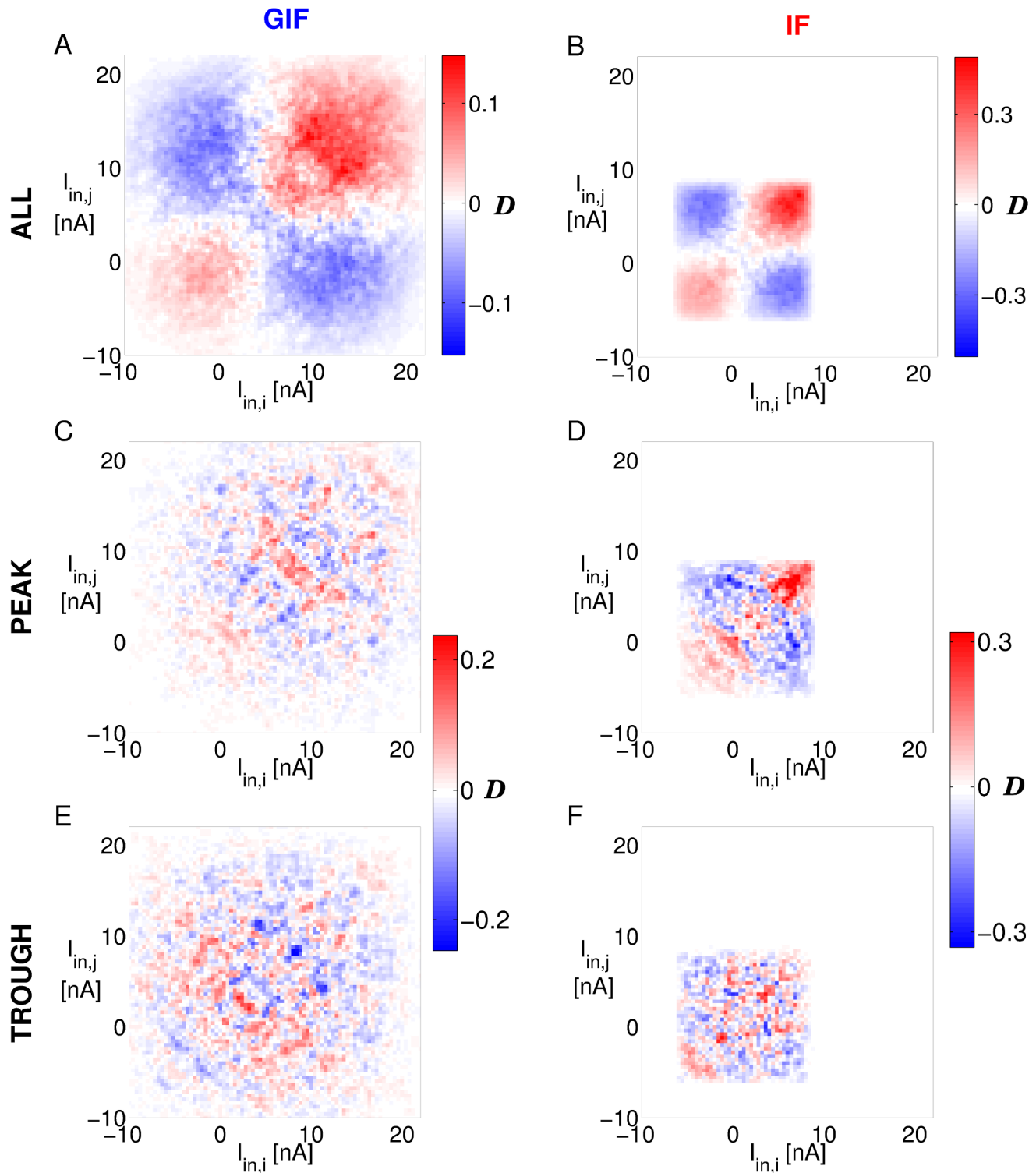
Figure 8. Deviation from independence of intrinsic currents for adjacent neurons. A: Deviation from independence \mathcal{D}(I_{in,i}, I_{in,j}) = \mathcal{P}(I_{in,i}, I_{in,j}) - \mathcal{P}^2(I_{in}) of intrinsic currents (I_{in,i}, I_{in,j}) flowing through the membrane of pairs (i, j) of adjacent neurons in the GIF network. Shades of red (blue) indicate (I_{in,i}, I_{in,j}) values that occur more (less) often than what expected under the assumption of independence. C, E: The same as A, but the probability density functions \mathcal{P}(I_{in,i}, I_{in,j}) and \mathcal{P}(I_{in}) are conditioned on the peak (C) or trough (E) of the mean I_{in} oscillation. B, D and F: The same as A, C and E, for the IF network. doi:10.1371/journal.pcbi.1003574.g008
