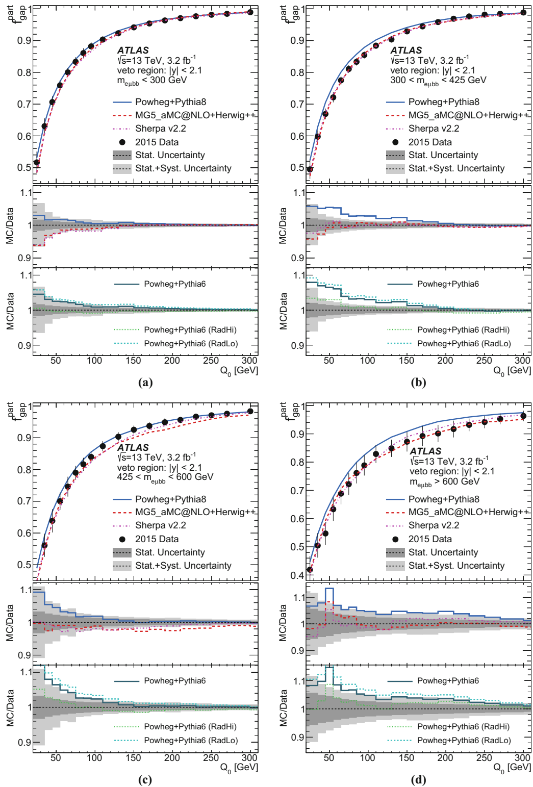
Fig. 14 The measured gap fraction f_m(Q_0) as a function of Q_0 in the full central veto region |y| < 2.1 for the invariant mass regions a m_{e\mu bb} < 300 GeV, b 300 < m_{e\mu bb} < 425 GeV, c 425 < m_{e\mu bb} < 600 GeV and d m_{e\mu bb} > 600 GeV. The data are shown by the points with error bars indicating the total uncertainty, and
