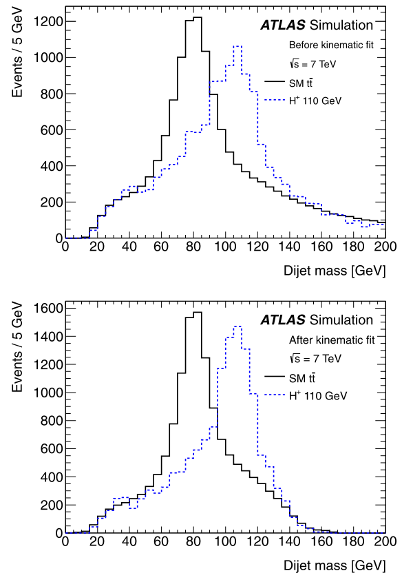
Fig. 2 Comparison of the dijet mass distribution before ( upper part ) and after ( lower part ) the kinematic fit and the \chi^2 < 10 selection criterion. The distribution is shown for MC simulations of SM t\bar{t} decays and the m_{H^+} = 110 GeV signal ( t\bar{t} \rightarrow H^+bW^-b ). The curves are normalised to the same area
