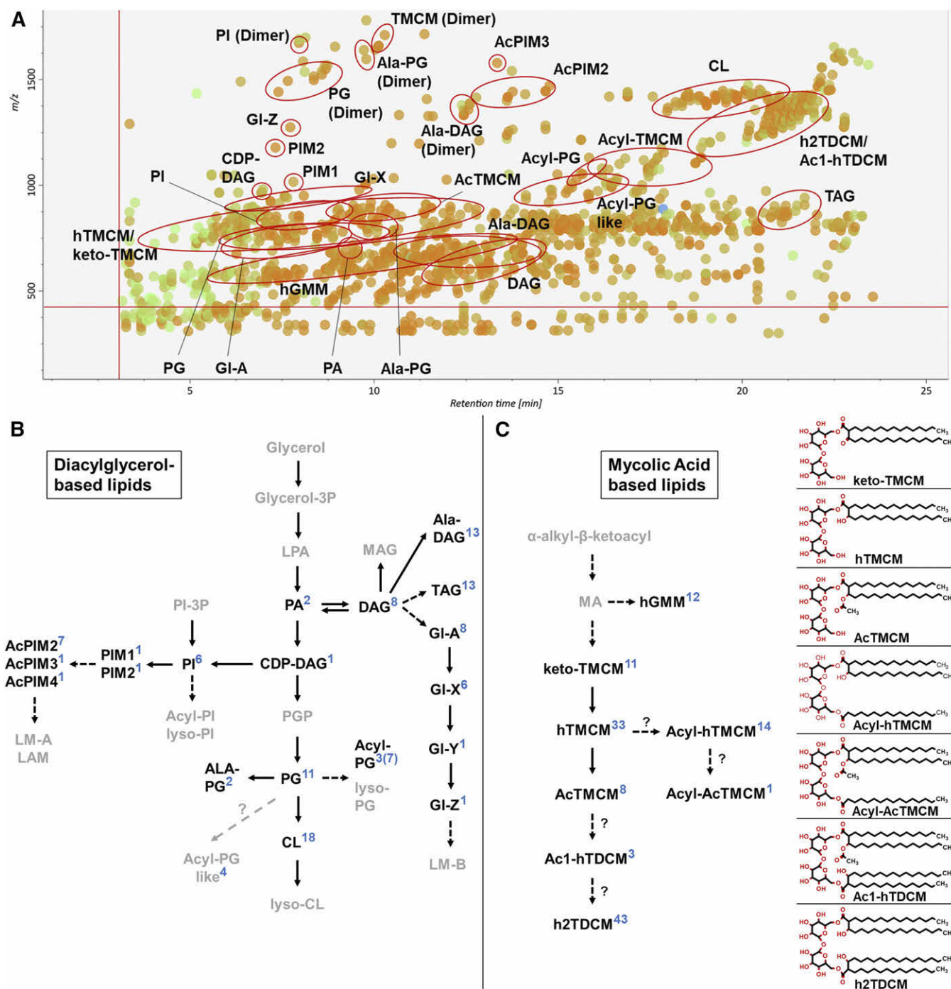
Fig. 1. LC-MS analysis of C. glutamicum lipids. A: MS/MS peak spot viewer of the C. glutamicum WT tTL fraction in MS-DIAL. The retention time (x axis) is plotted against the mass/charge ratio (y axis). Blue spots represent peaks of lower abundance based on peak area, green of intermediate abundance, and red of high abundance. A total of 174 lipid species (26 subclasses) were detected in the TL fraction of WT C. glutamicum . Each lipid (sub)class is highlighted with a red circle in the peak spot viewer of the MS-DIAL software. Note that not every spot within a circle belongs to the lipid (sub)class. B, C: Overview of pathways involved in DAG-based (B) and MA-based (C) lipid biosynthesis. Lipid (sub)classes identified via LC-MS/MS ESI QTOF in positive ionization mode using the established lipid libraries in MS-DIAL are in bold. The number of identified species in each lipid (sub)class are indicated in blue. Altogether, 233 lipids across 28 lipid (sub)classes were identified in the different C. glutamicum strains analyzed (WT, \Delta tmaT , and the \Delta tmaT complementation strain) and in the pooled biological quality control (PBQC); 108 were DAG-based and 125 MA-based lipids. The chemical structures of trehalose-containing MAs are shown.
