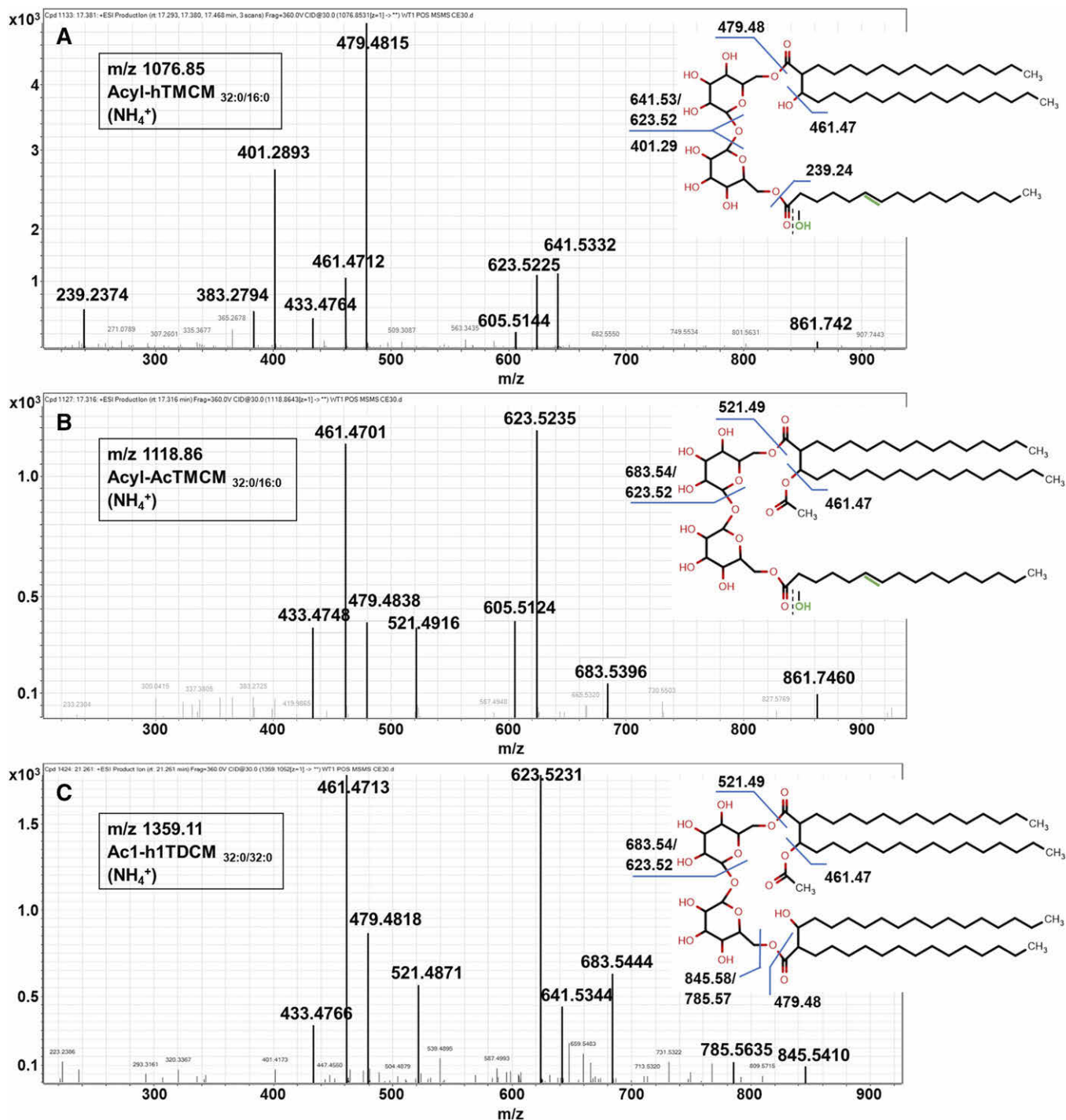
Fig. 2. Putative MS/MS fragmentation pattern of the three newly identified trehalose MAs. Fragmentation pattern of Acyl-hTMCM _{32:0/16:0} (A), Acyl-AcTMCM _{32:0/16:0} (B), and Ac1-h1TDCM _{32:0/32:0} (C). Altogether, 18 novel lipid species, comprising 14 Acyl-hTMCM, 1 Acyl-AcTMCM, and 3 Ac1-h1TDCM species, were detected. The FA moiety of Acyl-hTMCM (A) and Acyl-AcTMCM (B) could either carry a keto group or a hydroxyl group. In the case of a hydroxyl group, the FA moiety is monounsaturated (highlighted in green).
