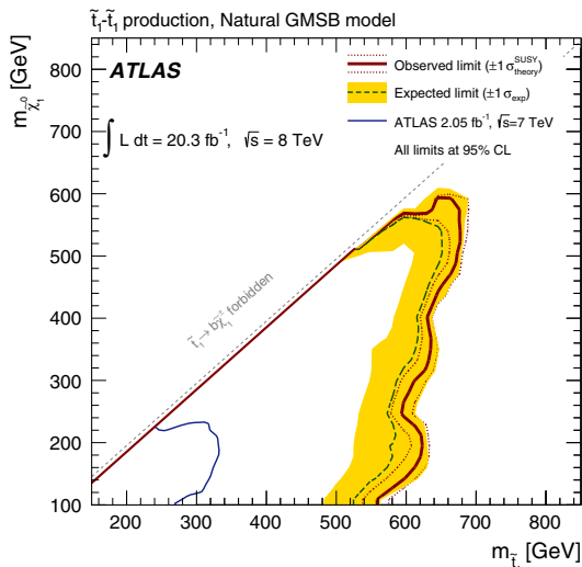
Fig. 6 Expected and observed exclusion limits at 95 % CL for the stop natural GMSB model described in the text. The contours of the band around the expected limit are the \pm 1\sigma results, including all uncertainties except theoretical uncertainties on the signal cross section. The dotted lines around the observed limit illustrate the change in the observed limit as the nominal signal cross section is scaled up and down by the theoretical uncertainty. For comparison, the observed exclusion limit with 2.05 \text{ fb}^{-1} of data at \sqrt{s} = 7 \text{ TeV} at ATLAS for a similar model [34] is shown
