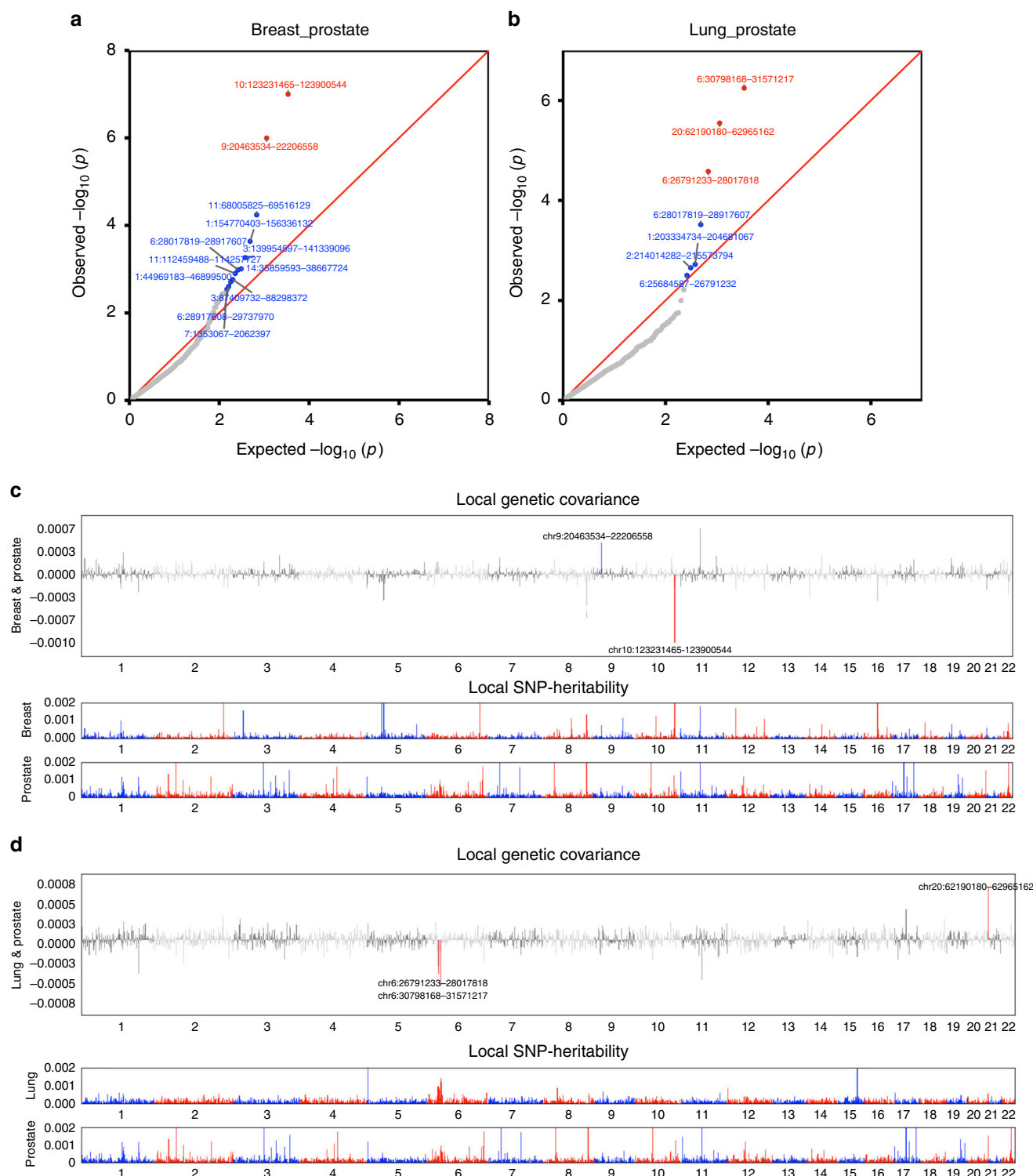
Fig. 2 Local genetic correlation between breast, lung and prostate cancer. The region-specific p -values for the local genetic covariance for breast and prostate cancer are shown in a , and for lung and prostate cancer in b . Each dot presents a specific genomic region. In the QQ plots, red color indicates significance after multiple corrections ( p < 0.05/1703 regions compared), and blue color indicates nominal significance ( p < 0.05/15 pairs of cancers compared). Manhattan-style plots showing the estimates of local genetic covariance for breast and prostate cancer ( c ), and for lung and prostate cancer ( d ). Although breast and prostate cancer only show modest genome-wide genetic correlation, two loci exhibit significant local genetic covariance. Similarly, albeit the negligible overall genetic correlation for lung and prostate cancer, three loci present significant local genetic covariance. In the Manhattan plots, red color indicates even number chromosomes and blue color indicates odd number chromosomes
