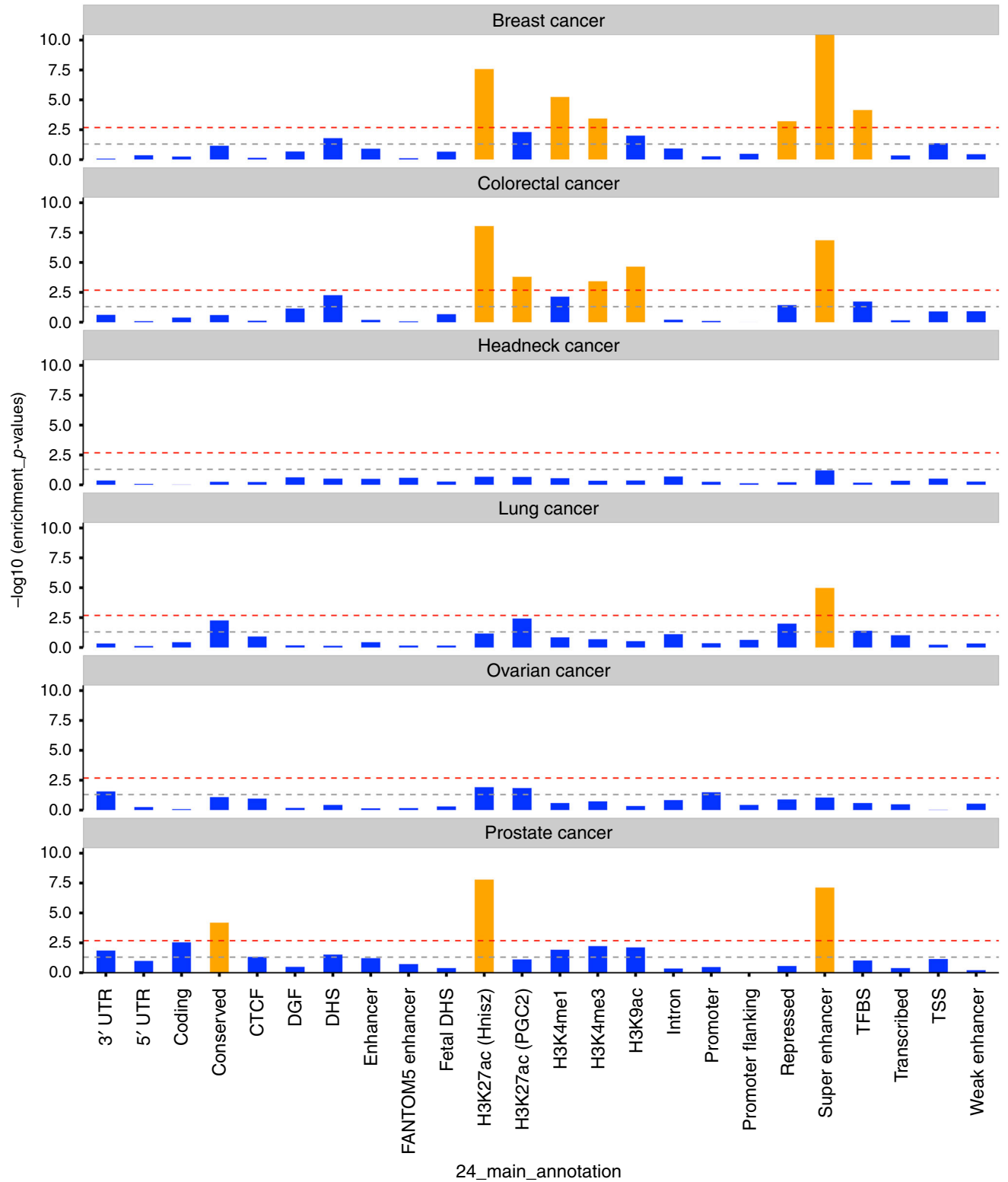
Fig. 5 Enrichment p -values of 24 non-cell-type-specific functional categories over six cancer types. The x-axis represents each of the 24 functional categories, y-axis represents log-transformed p -values of enrichment. Annotations with statistical significance after Bonferroni corrections ( p < 0.05/24 ) were plotted in orange, otherwise blue. The horizontal gray dash line indicates p -threshold of 0.05; horizontal red dash line indicates p -threshold of 0.05/24. From top to bottom are six panels representing six cancers: breast cancer, colorectal cancer, head/neck cancer, lung cancer, ovarian cancer, and prostate cancer. TSS transcription start site, UTR untranslated region, TFBS transcription factor binding sites, DHS DNase I hypersensitive sites, DGF digital genomic foot printing, CTCF CCCTC-binding factor
