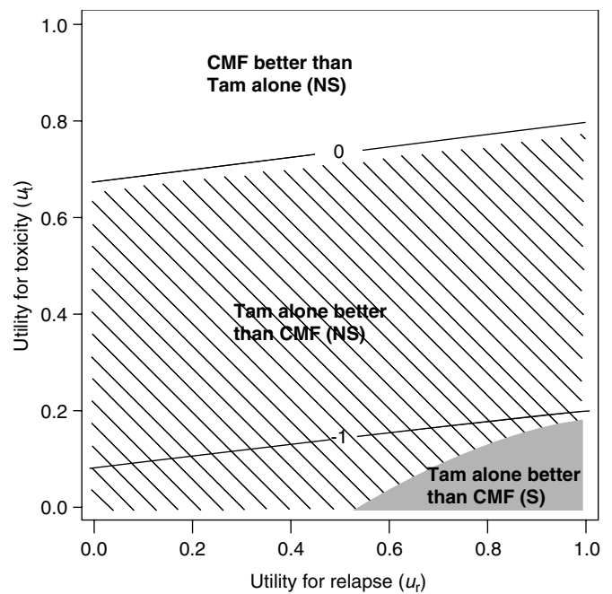
Figure 7 Threshold utility analysis of the ER-positive cohort ( N = 1217 ). The diagonal lines indicate the units of months gained in Q-TWiST for different utilities for Tox and Rel. The utilities for TWiST is defined as u_{twist} = 1 (i.e. reference state). The solid line labelled 0 is the threshold above which CMF followed by Tam results in improved Q-TWiST. The area below 0 with hatch marks represents improved Q-TWiST for Tam alone. The shaded region (bottom right) represents utilities ( u_t and u_r ) for which the improvement in Q-TWiST is statistically significant for Tam alone ( P \leq 0.05 ). S = significant and NS = not significant.
