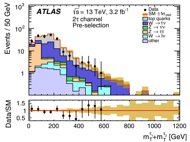
(b) m_{T1}^{\tau} + m_{T2}^{\tau} distribution in the 2\tau channel
