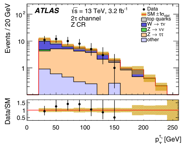
(b) Z(\tau\tau) +jets CR
