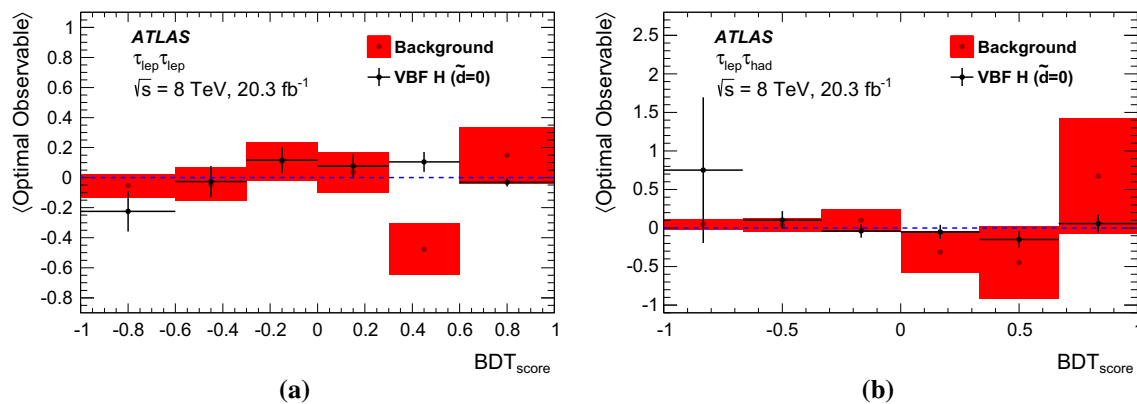
Fig. 2 Mean of the Optimal Observable as a function of the \text{BDT}_{\text{score}} for the SM signal (black dots with error bars) and for the sum of all background processes (filled red area), for the a \tau_{\text{lep}}\tau_{\text{lep}}
