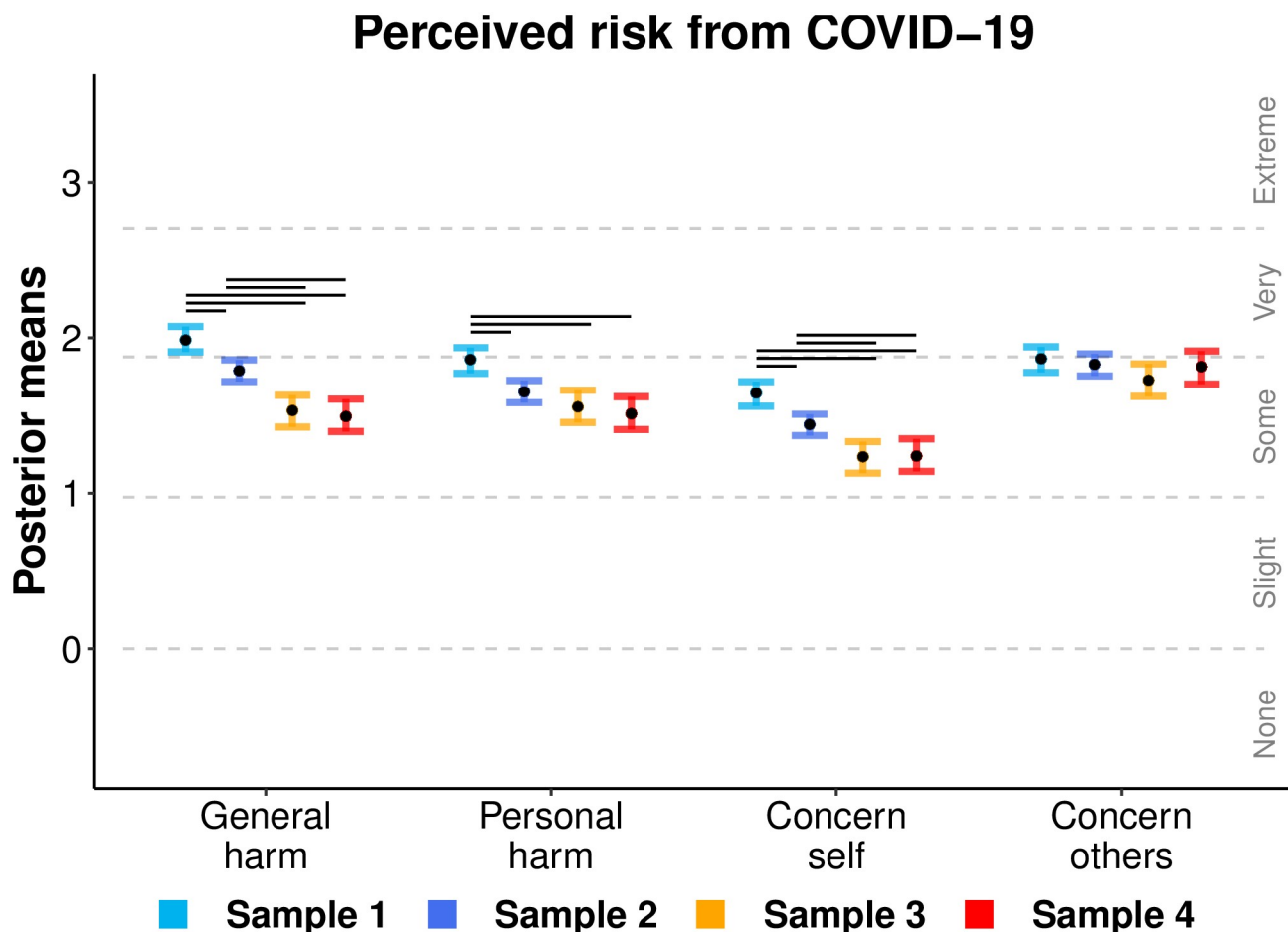
Fig 4. Ordinal regression mean posterior distributions for items assessing the perceived risk from COVID-19 for each sample. Black points display mean point estimates and coloured error bars display the 95% highest posterior density interval thereof. Dotted lines indicate the ordinal regression threshold parameters which separate the continuous latent variables into the ordinal response categories made by participants ('None' to 'Extremely'). Non-overlapping intervals (within items) are denoted by horizontal bars above each comparison.
