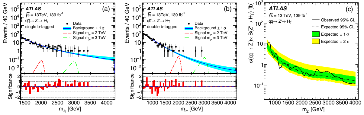
FIG. 1. (a),(b) Distribution of the reconstructed m_J in the single- and double- b -tagged categories, with the background-only fits shown by the solid lines. The corresponding chi-square probabilities of the fits are 46% and 23%, after rebinning requiring at least five events in each bin. Hypothetical signal distributions for m_{Z'} = 2 TeV and m_{Z'} = 3 TeV with arbitrary normalizations are plotted for illustration purposes. The bottom panel gives the significance (deviation/statistical uncertainty) for each bin, calculated using the recommendation of Ref. [55]. The impact on the background fit from the statistical uncertainties of BPDF parameters is shown as a light band around the solid line. This effect is incorporated into the significance calculation. (c) Observed and expected 95% confidence-level limits on \sigma \times \mathcal{B} as a function of m_{Z'} .
