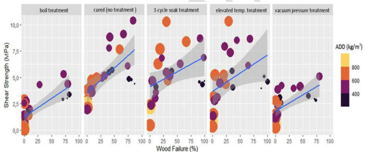
Figure 5: Showing the effect of air-dry density (ADD) on shear strength and wood failure of all the tested species across the different exposure conditions.
