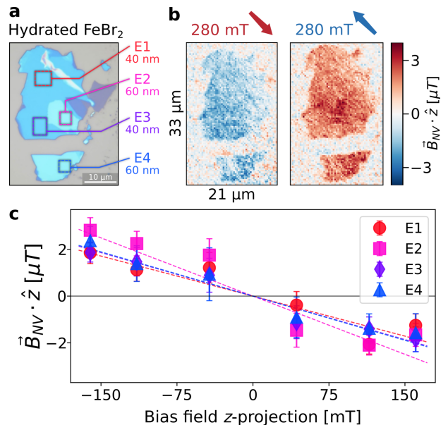
FIG. 5. Diamagnetic behavior in hydrated \text{FeBr}_2 sample. (a) Optical image in which several regions are identified and labeled according to their height. (b) Reconstructed stray field maps measured at 4 K and projected along the z axis for opposite 280 mT (left) and -280 mT (right) bias fields applied along the (-1,1,-1) NV axis. (c) Average stray fields vs bias fields, both projected along the z axis, for all identified regions (error bars represent one standard deviation uncertainty). A proportional and opposite response relative to the bias field can be observed in all regions, consistent with diamagnetism.
