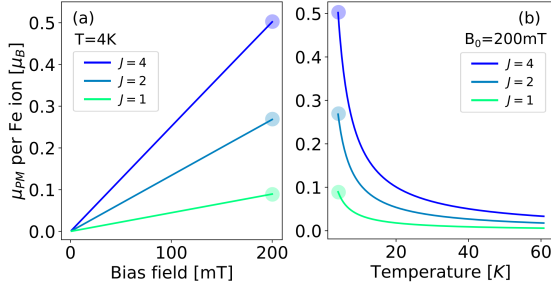
FIG. 11. Calculated paramagnetic moment per Fe ion (in Bohr magneton units) as a function of: (a) bias field at 4 K and (b) temperature at 200 mT. The values at 4 K and 200 mT have been identified with shaded circles in both plots.
