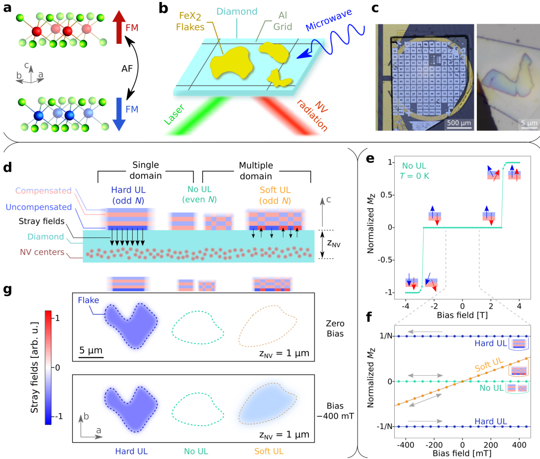
FIG. 1. Experimental setup and expectations for antiferromagnetic flakes. (a) Crystallographic scheme for iron halides structures: the \text{Fe}^{2+} ions (blue and red) are ferromagnetically coupled within a layer, and each layer is antiferromagnetically coupled with the adjacent ones. Magnetic contributions from the halogen ions (green) are negligible. (b) Widefield magnetometry experimental setup: the samples lie on top of a diamond substrate, which is patterned with an aluminum grid and an omega-shape gold resonator for microwave (MW) delivery. A green laser beam illuminates the diamond from below and the NV radiation is collected by a sCMOS camera. (c) Optical images of (left) the diamond substrate, where the MW resonator and aluminum grid can be seen, and (right) a \text{FeBr}_2 thin flake covered by a hBN flake. (d) Side view scheme of the thin flakes lying on top of the diamond, according to the different models from left to right: hard uncompensated layer (“Hard UL”) for single domain configuration, “No UL” for both single and multiple domains and “Soft UL” for multiple domains. The generated stray fields are sensed by a dense layer of NV spin defects at a standoff distance z_{\text{NV}} below the top surface. (e) Simulated hysteresis cycle at zero absolute temperature of the z -projected magnetization (normalized to the saturation value) as a function of the bias field applied along the c axis, for an iron halide flake with N layers according to the No UL model in the single domain configuration. The schemes show the magnetization orientation of the sublattices at different stages. (f) Zoom-in version of the previous plot for our bias field measurement range, showing the models No UL (green), Hard UL (blue) and Soft UL (orange). The arrows indicate the sweeping bias field direction. (g) Simulated stray fields for arbitrary flakes’ geometries under zero bias (top panel) and -400 mT bias field (bottom panel). Each column corresponds to a different model from left to right: Hard UL, No UL and Soft UL.
