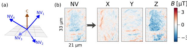
FIG. 13. (a) Orientation of the four NV axes relative to the crystal anisotropy c axis. (b) Full stray field vector reconstruction from the original map measured along the \text{NV}_2 axis at 280 mT bias field (left), projected along the (x,y,z) directions (right).
