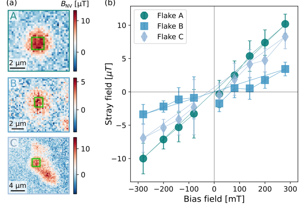
FIG. 10. Stray field hysteresis measurements for different flakes. (a) Stray field maps at 280 mT bias fields for three flakes named A, B, C (from top to bottom) in which the stray fields are averaged within the green delimited region. (b) Stray vs bias fields, cycling the bias field from zero to the maximum positive value, then to the maximum negative value and finally back to zero. All flakes show negligible magnetization and coercivity.
