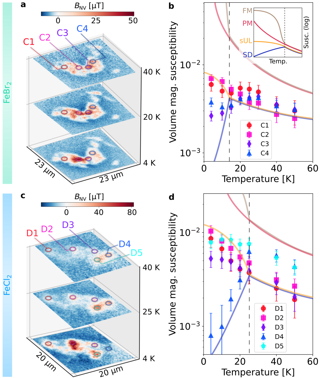
FIG. 4. Volume susceptibility versus temperature along with models expectations. (a,c) Stray field maps under 200 mT bias along the c axis, at temperatures below, close and above the Néel temperature. The color scale represents the field intensity sensed by the NV sensors at 500 nm (FeBr 2 ) and 250 nm (FeCl 2 ) standoff distance. (b,d) Averaged volume magnetic susceptibility as a function of temperature for identified regions (error bars represent one standard deviation) along with expectations according to different models (solid lines): Single Domain antiferromagnetism (blue), Soft Uncompensated Layer (orange), Paramagnetism (red) and Ferromagnetism (brown). The inset in (b) shows the qualitative behaviors of these models in a larger scale, valid for both samples. The Néel temperature is represented by a vertical dotted line.
