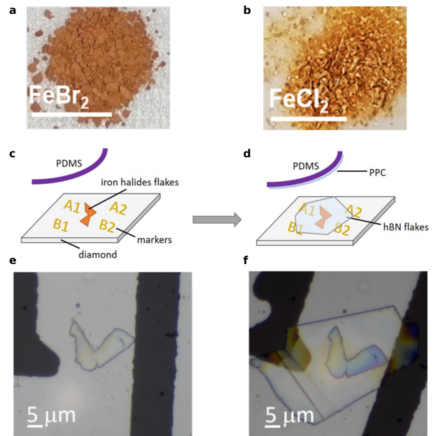
FIG. 6. (a) \text{FeBr}_2 and (b) \text{FeCl}_2 bulk powders used for direct mechanical exfoliation, each scale bar is 5 mm long. (c,d) Schematic sealing process in which thin iron halides flakes are covered by a protective hBN flake (thickness < 40 \text{ nm} ). (e,f) Optical images for a \text{FeBr}_2 flake at the c,d stages, respectively.
