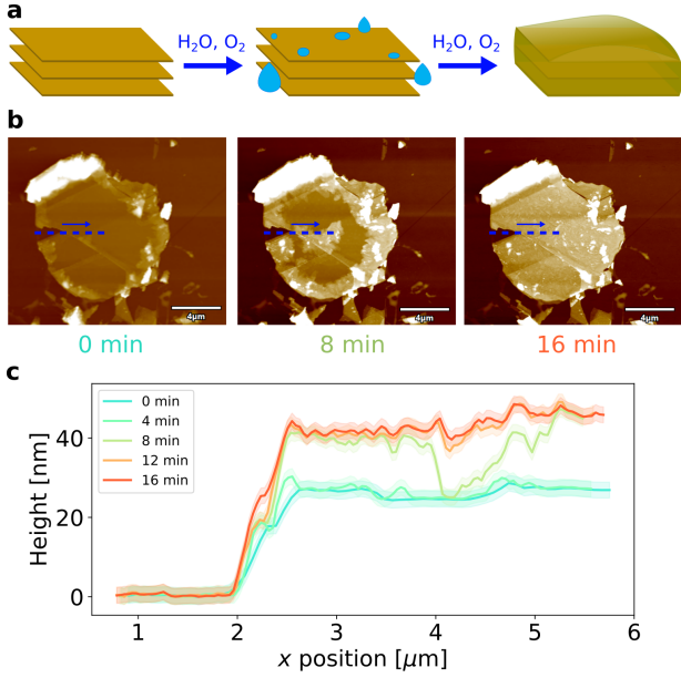
FIG. 12. Hydration process in a \text{FeBr}_2 flake exposed to ambient conditions. (a) Hydration scheme: the sample is introduced to ambient conditions ( \text{H}_2\text{O} and \text{O}_2 ) and it progressively becomes hydrated, enlarging its volume. (b) AFM images at different stages of the process, starting from a protected \text{N}_2 atmosphere at ‘0 min’ and evolving in the presence of air until ‘16 min’. No noticeable changes occurred after that time. (c) Height profiles across the dotted line at different times, showing how the thickness increased as a result of hydration. The thicker regions of the flake were much easier to degrade than the thinner regions.
