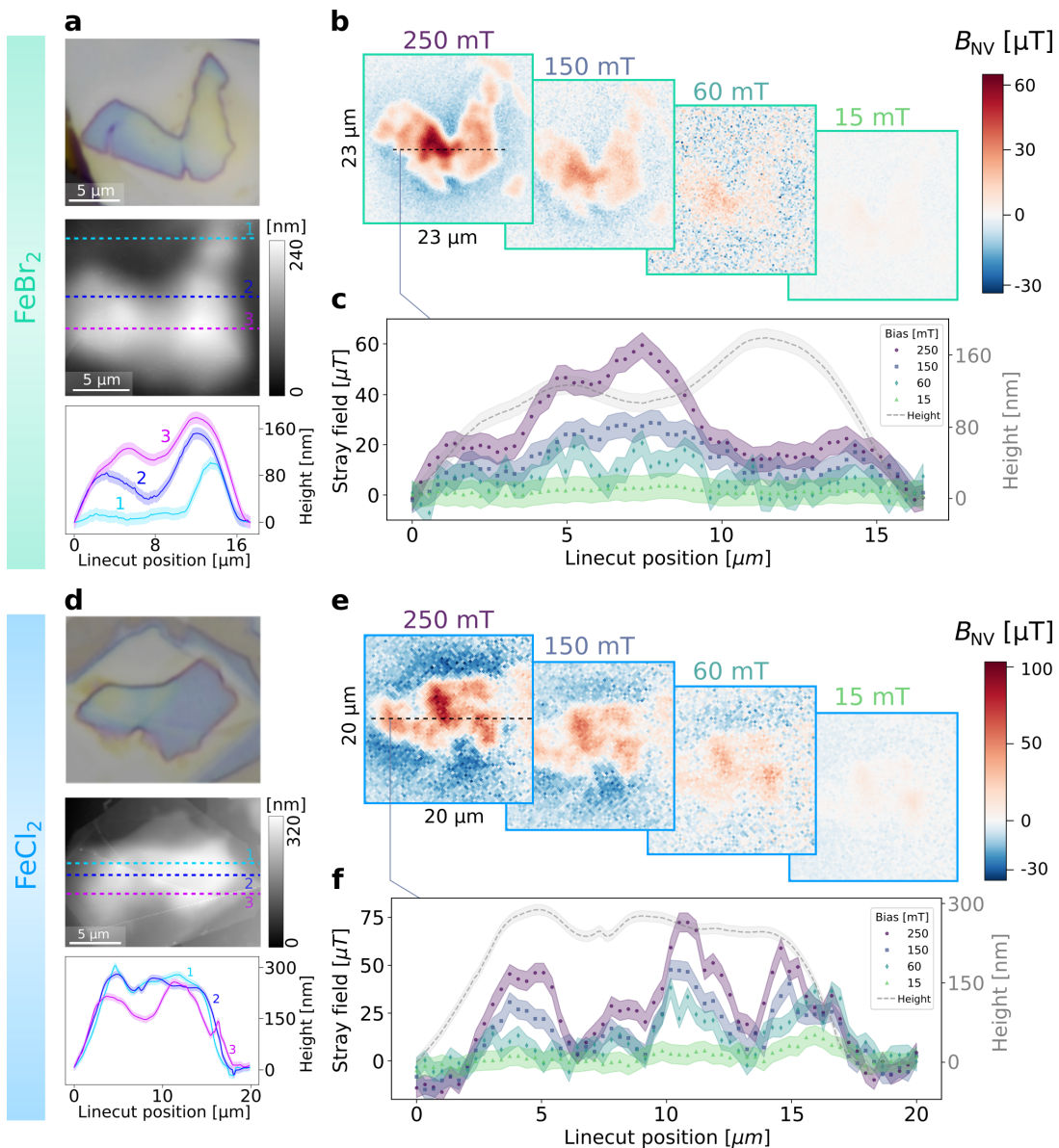
FIG. 2. Samples characterization and magnetic maps showing negligible remanent magnetization. (a),(d) Optical and AFM characterization for FeBr 2 and FeCl 2 samples, respectively. Optical images (top panels) match the AFM measurements (middle panels), in which linecuts are correlated with height profiles (bottom panels, shaded areas represent experimental uncertainties). (b),(e): Stray field map series for FeBr 2 and FeCl 2 samples, respectively, under different bias fields. For both samples, the magnetic signal decreases with the bias field, pointing to zero or very low remanent magnetization. (c),(f): Stray fields and height profiles along the linecuts shown in b,e for FeBr 2 and FeCl 2 samples, respectively, evidencing no correlation with the samples' topographies.
