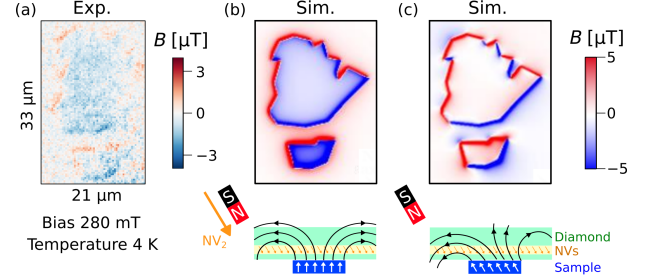
FIG. 14. (a) Experimental \text{NV}_2 -projection of the stray fields generated by a \text{FeBr}_2 flake under a 280 mT bias field applied along the \text{NV}_2 axis at 4 K, sensed by the \text{NV}_2 centers at 500 nm standoff distance. (b,c) Stray field \text{NV}_2 -projections simulated under the same bias and temperature conditions assuming (b) a strong anisotropy c axis and (c) no anisotropy axis.
