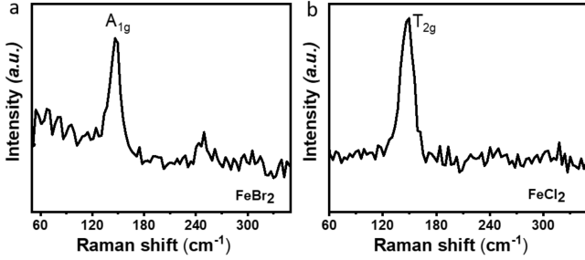
FIG. 8. Raman evaluation for main samples (a) \text{FeBr}_2 and (b) \text{FeCl}_2 . The main vibrational modes A_{1g} of \text{FeBr}_2 and T_{2g} of \text{FeCl}_2 are clearly present and provide evidence that the samples were not degraded.
