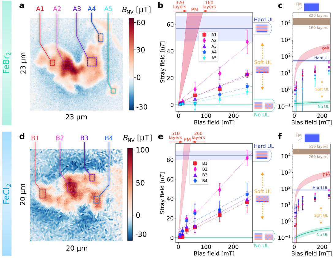
FIG. 3. Magnetic signal versus bias field along with possible magnetic models. (a,d) Stray field maps at temperature 4 K and bias 200 mT along the c axis. The color scale represents the field intensity sensed by the NV sensors at 500 nm (FeBr 2 ) and 250 nm (FeCl 2 ) standoff distance. (b,e) Averaged stray fields as a function of bias field for identified regions (error bars represent one standard deviation) along with expectations for the different models: No Uncompensated Layer (green solid line), Hard Uncompensated Layer (blue solid line, the shaded area represents one standard deviation), Soft Uncompensated Layer, which represents a region in-between as depicted by the right-margin schemes, and Paramagnetic (red shaded area). Dashed curves are linear fits for experimental points. (c,f) Same plots but using logarithmic scale for stray fields and including the ferromagnetic model (brown shaded area).
