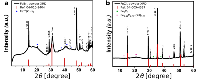
FIG. 9. X-Ray Diffraction for bulk (a) \text{FeBr}_2 and (b) \text{FeCl}_2 materials before mechanical exfoliation. The experimental patterns (black) are compared with peak positions of reference powder patterns (red vertical lines) to show that they share the same crystal structure ( P\bar{3}m1 ).
