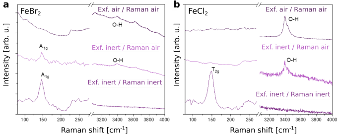
FIG. 7. (a) \text{FeBr}_2 and (b) \text{FeCl}_2 thin flakes’ stability studied by Raman spectroscopy under different preparation and evaluation conditions: both exfoliation and Raman control in air (top panels), exfoliation in glovebox and Raman control in air (middle panels) and exfoliation in glovebox and Raman control in hermetic cell (bottom panels). Characteristic vibrational modes of \text{FeBr}_2 ( A_{1g} ) and \text{FeCl}_2 ( T_{2g} ) structures are clearly present in the most protected conditions, and they gradually disappear when samples are exposed to air. Consistently, water molecule vibrations (O-H, around 3400\text{ cm}^{-1} ) only appear when the samples are exposed to air.
