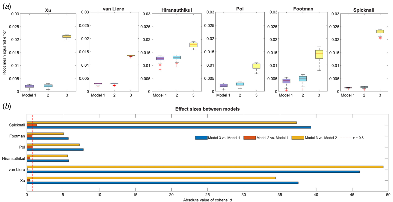
Fig. 2. Root mean squared error and effect size of calibrated models with or without masturbation across six different datasets. (a) The boxplots of root mean squared error. (b) The effect size of calibrated models. Effect sizes were classified as small (Cohen’s d = 0.2 ), medium (Cohen’s d = 0.5 ), and large (Cohen’s d \geq 0.8 ). Model 1: anal sex, oral sex, rimming, kissing, and sequential sexual practices; Model 2: Model 1 + masturbation; Model 3: sequential sexual practices + masturbation.
