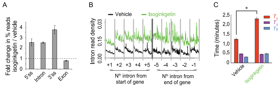
Figure 3. The rate of lariat formation is decreased two-fold by isoginkgetin treatment. (A) Genome-wide expression of 5' splice sites, 3' splice sites, and introns are increased relative to exons upon treatment of HeLa cells with isoginkgetin (30 \mu M, 18 hours), based on total RNA-Seq (dUTP method [18], Illumina). The height of each bar indicates the fold change, from vehicle- to isoginkgetin-treated cells, in the mean fraction of reads aligning to each genic feature ( p < 0.02 from two-tailed t -tests for all ratios). (B) Isoginkgetin treatment increases the "guillotine" base height ( p = 10^{-12} ) of intronic expression without increasing the blade height ( p = 0.5 ), consistent with a splicing defect (compare to Fig. 1A). Only introns longer than 50 kb from genes with at least 10 introns are included in these meta-intron profiles, which show the last 50 kb of each aggregated intron. Introns of different lengths are aligned at their 3' ends. RNA-Seq density is normalized as read counts per 10M uniquely aligning reads. The indicated values are from an average of three biological replicates, and p -values are from two-tailed t -tests based on mean values for aggregated introns 2–10 ( n = 9 ). (C) Isoginkgetin treatment leads to a decreased rate of lariat formation (* indicates p = 0.02 ) without affecting exon ligation or excised lariat degradation ( p = 0.22, 0.08 ), with calculations as in Fig. 1. p -values are from two-tailed t -tests with n = 3 biological replicates. Error bars in (A, C) represent s.e.m. from three biological replicates. doi:10.1371/journal.pone.0089673.g003
