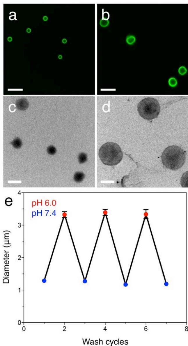
Figure 1. Non-covalently stabilized PDPA C12 capsules obtained from 2.6 μm-diameter silica templates, as observed by a) and b) fluorescence microscopy (PDPA C12 capsules labeled with AF488), and c) and d) TEM at pH 7.4 (left column) and pH 6.0 (right column). Scale bars are 5 μm. e) Diameters of PDPA C12 capsules in response to alternate pH wash cycles. The diameters of 20 capsules were sized using a fluorescence microscope.
