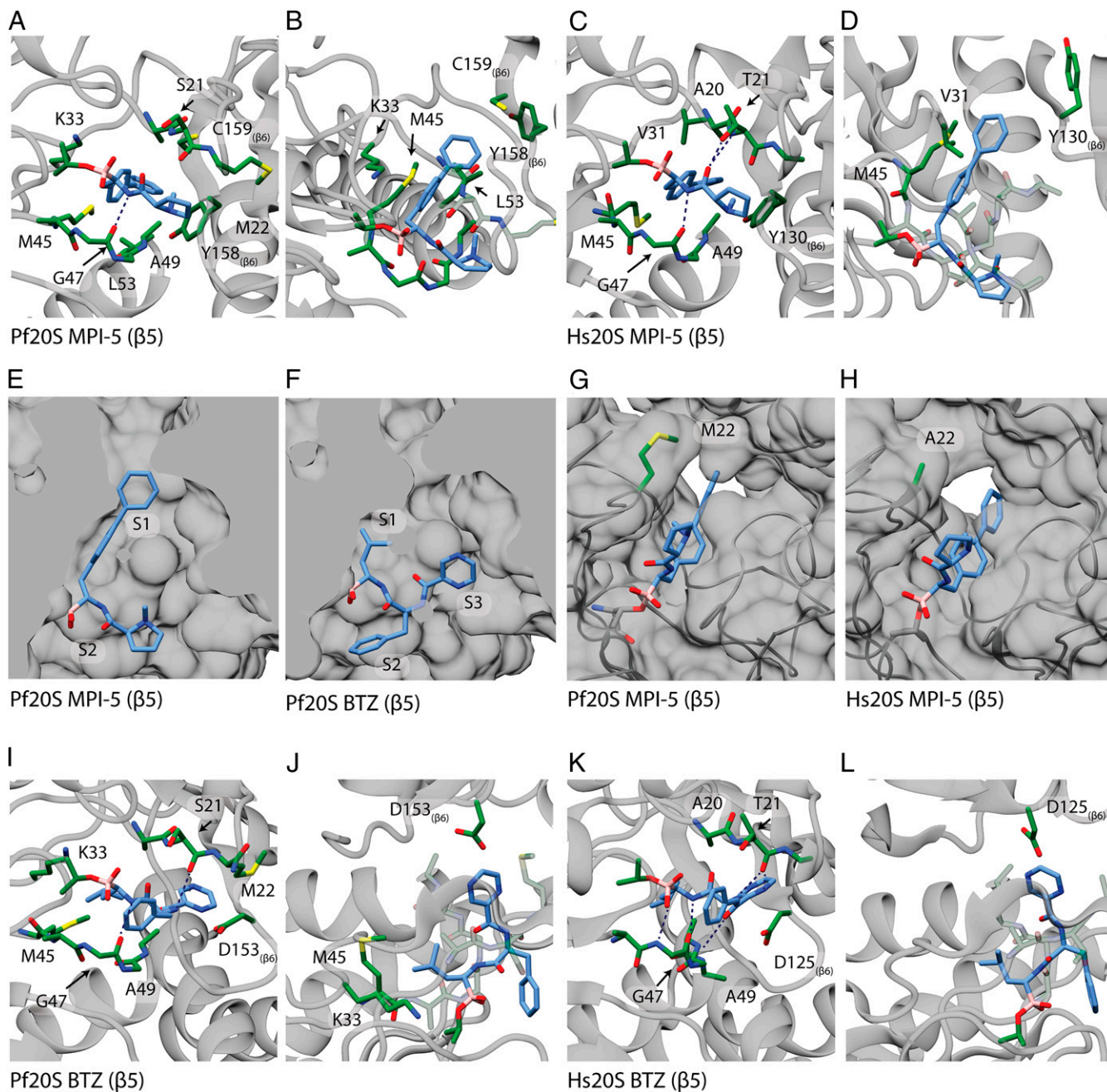
Fig. 3. Structures of Pf20S and Hs20S \beta 5 active sites with bound MPI-5 or bortezomib. Pf20S \beta 5 (A and B) and Hs20S \beta 5c (C and D) are shown as side (A and C) and top (B and D) views, with interacting residues (green) around the covalently bound MPI-5 (blue). (E and F) Cut-away showing solvent-accessible surface of the Pf20S \beta 5 active site illustrating the different poses adopted by MPI-5 (E) and bortezomib (F). Substrate binding pockets, S1, S2, and S3 are marked. (G and H) Met22 creates a hydrophobic ledge over the ligand binding site in Pf20S \beta 5 , while Ala22 permits more solvent access in the Hs20S \beta 5c active site around the covalently bound MPI-5. Pf20S \beta 5 (I and J) and Hs20S \beta 5c (K and L) are shown as side (I and K) and top (J and L) views, with interacting residues (green) around the covalently bound bortezomib (blue).
