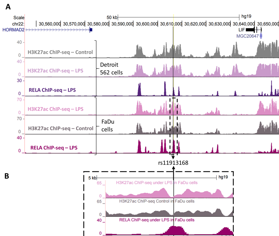
Figure 2. Genomic data for rs11913168. RELA and H3K27ac ChIP-seq data following LPS stimulation of Detroit 562 and FaDu cells are represented. The SNP of interest is indicated with a black line. The lower panel (B) consists of a magnification of the dashed box in the upper panel (A).
