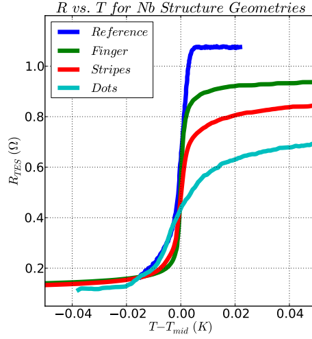
Figure 2. Effect of Nb structures on the R(T) profile of prototype TESs. The “reference” sample is a plain MoAu bilayer TES. The “finger” pattern was a bar 11\text{ }\mu\text{m} wide that completely bisected the TES across its middle, perpendicular to the direction of current flow. The “zebra stripes” were a series of 11\text{ }\mu\text{m} wide parallel bars partially spanning the TES. Our final design was the “dots” arrangement of 3\text{ }\mu\text{m} diameter dots spaced 11\text{ }\mu\text{m} apart.
