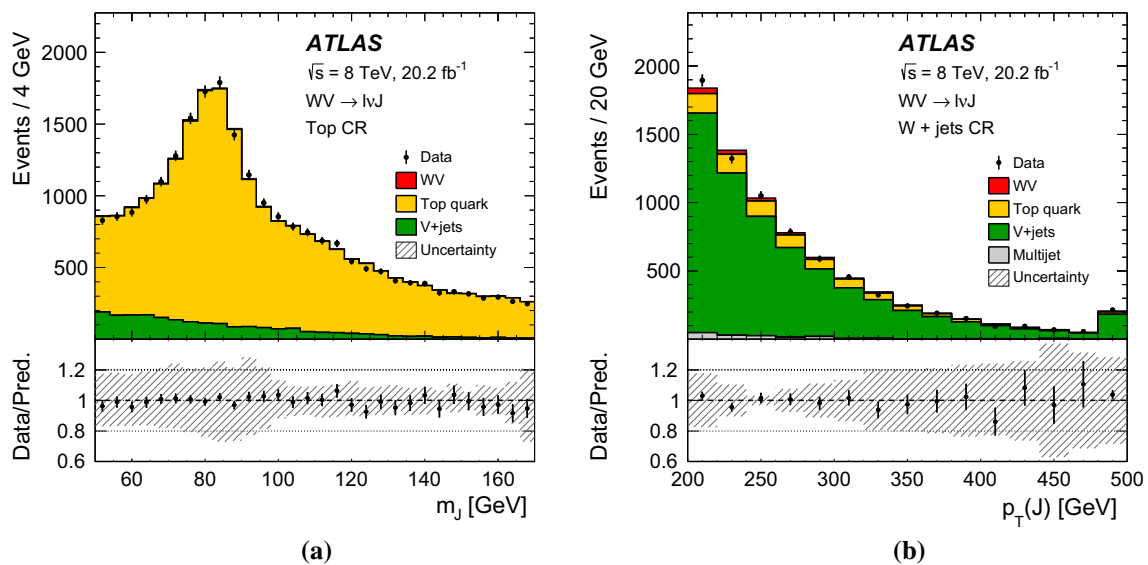
Fig. 3 Comparison between data and prediction in the WV \rightarrow \ell\nu J channel for a m_J in the top CR, and b p_{T(J)} in the W + jets CR. A scale factor is applied to the top-quark background prediction in the top CR and the W + jets CR, and a scale factor is applied to the W + jets
