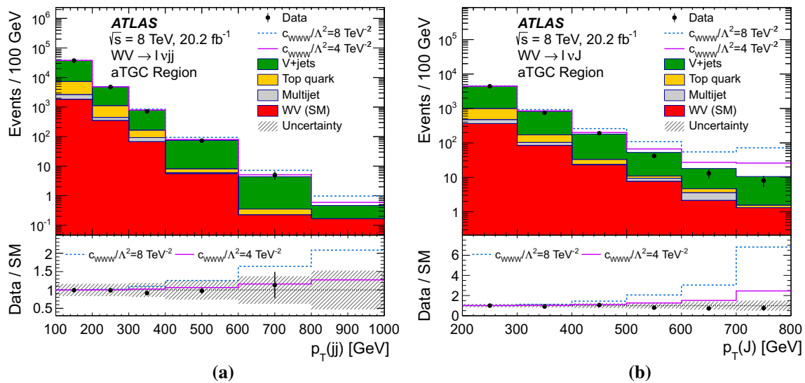
Fig. 7 The observed a p_T(jj) distribution in the WV \rightarrow \ell v jj aTGC signal region, and b p_T(J) distribution in the WV \rightarrow \ell v J aTGC signal region, overlaid with the background and signal prediction. The expected BSM enhancements due to anomalous values of the EFT parameter c_{WWW}/\Lambda^2 are also shown, for c_{WWW}/\Lambda^2 = 4 \text{ TeV}^{-2} and
