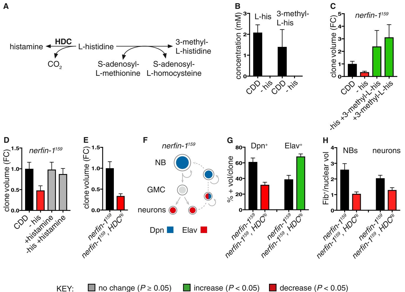
Figure 2. Histidine metabolic perturbations affect nerfin-1 neuron-to-NB reversion.
