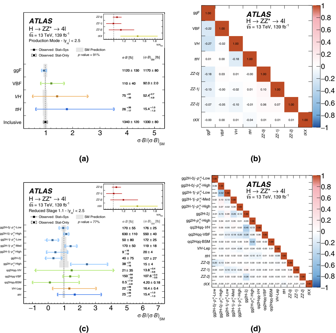
Fig. 10 The observed and expected SM values of the cross-sections \sigma \cdot \mathcal{B} normalised by the SM expectation (\sigma \cdot \mathcal{B})_{\text{SM}} for (a) the inclusive production and in the Production Mode Stage and (c) the Reduced Stage-1.1 production bins for an integrated luminosity of 139 \text{ fb}^{-1} at \sqrt{s} = 13 TeV. The fitted normalisation factors for the ZZ and tXX background are shown in the inserts. Different colours indicate dif-
