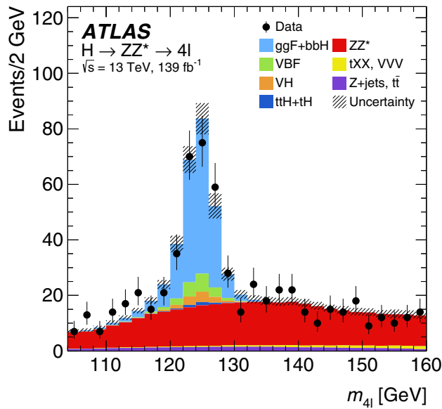
Fig. 5 The observed and expected (post-fit) four-lepton invariant mass distributions for the selected Higgs boson candidates, shown for an integrated luminosity of 139 \text{ fb}^{-1} at \sqrt{s} = 13 \text{ TeV} . The SM Higgs boson signal is assumed to have a mass m_H = 125 \text{ GeV} . The uncertainty in the prediction is shown by the hatched band, calculated as described in Sect. 7. For comparison only, the hatched band includes the theoretical uncertainties in the SM cross-section for the signal and the background processes
