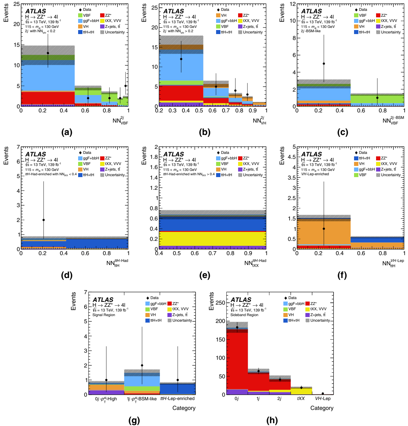
Fig. 8 The observed and expected NN output (post-fit) distributions for an integrated luminosity of 139 \text{ fb}^{-1} at \sqrt{s} = 13 \text{ TeV} in the different categories: (a) NN_{VBF} in 2j with NN_{VH} < 0.2 , (b) NN_{VH} in 2j with NN_{VH} > 0.2 , (c) NN_{VBF} in 2j -BSM-like, (d) NN_{tH} in ttH -Had-enriched with NN_{tXX} < 0.4 , (e) NN_{tXX} in ttH -Had-enriched with NN_{tXX} > 0.4 and (f) NN_{tH} in VH -Lep-enriched. g Shows the categories where no NN discriminant is used while (h) shows the sidebands
