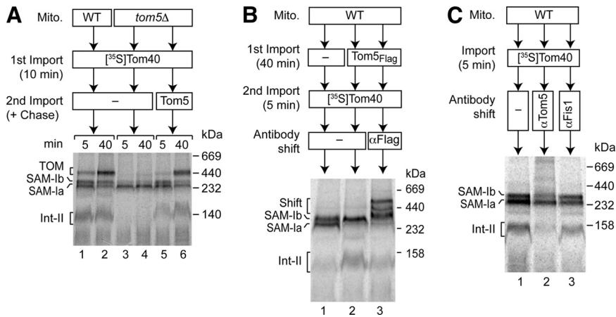
Figure 4. Tom5 is a component of the SAM-Ib intermediate of Tom40 assembly. (A) ^{35}\text{S} -labeled Tom40 was imported for 10 min into wild-type (WT) and tom5 \Delta mitochondria. Subsequently, mitochondria were reisolated and a chase reaction was performed in the absence or presence of chemical amounts of Tom5 for the indicated periods. The assembly of ^{35}\text{S} -labeled Tom40 was analyzed by blue native electrophoresis and autoradiography. (B) Chemical amounts of Tom5 Flag were imported into wild-type mitochondria. After reisolation of the mitochondria, ^{35}\text{S} -labeled Tom40 was imported for 5 min, the mitochondria were lysed, and anti-Flag antibodies were added. The assembly of Tom40 and antibody shifts were analyzed by blue native electrophoresis and autoradiography. (C) ^{35}\text{S} -labeled Tom40 was imported into wild-type mitochondria. Subsequently, antibody shift assays with the indicated antibodies were performed.
