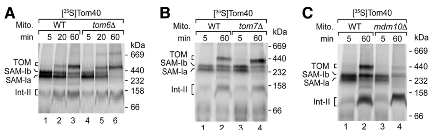
Figure 5. Analysis of SAM-Ib formation in mitochondria lacking Tom6, Tom7, or Mdm10. ^{35}\text{S} -labeled Tom40 was imported for the indicated periods into mitochondria isolated from (A) tom6 \Delta , (B) tom7 \Delta , or (C) mdm10 \Delta yeast strains. The assembly of Tom40 was analyzed by blue native electrophoresis and autoradiography.
