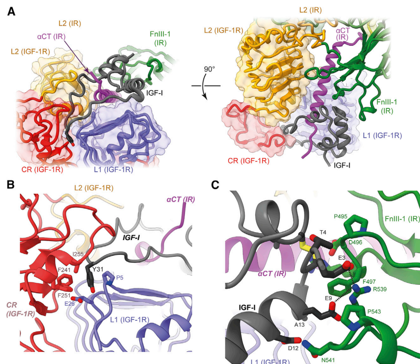
Figure 3. Detail of the structure of [IGF-II]-complexed HybZip
