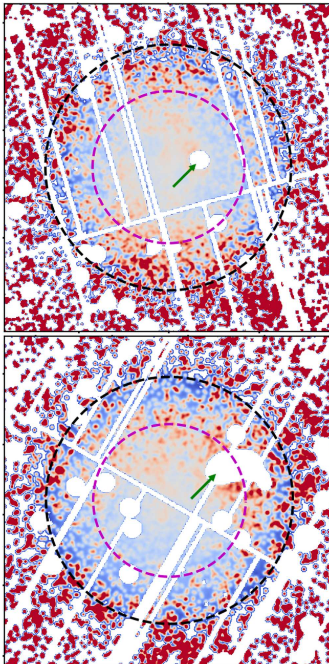
Figure 9. The \delta S / \delta I_{\text{ICM}} image for SPT-CLJ0658-5556 (top) and SPT-CLJ0014-3022 (bottom) as seen with the pn camera (400–1250 eV). The substructures masked are indicated with green arrows; other masked regions are from point sources and chip gaps.
