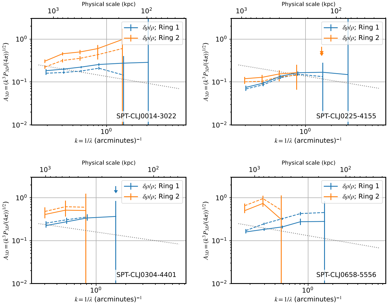
Figure 10. The resultant amplitude spectra, A_{\rho} , for clusters with substructure masked (solid lines) and unmasked (dashed lines). The clusters are SPT-CLJ0014-3022 (top left), SPT-CLJ0225-4155 (top right), SPT-CLJ0304-4401 (bottom left), and SPT-CLJ0658-5556 (bottom right). Arrows indicate a 3\sigma upper limit.
