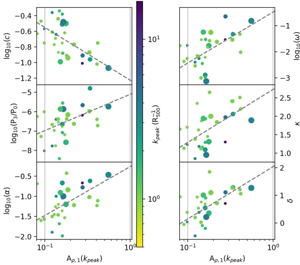
Figure 2. Scatter plots of dynamical parameters relative to the inferred A_\rho in Ring 1. Sizes of markers indicate the maximal \xi (see Appendix A) in A_{\rho,1} . The coloring of the markers corresponds to the location (wavenumber) of the inferred peak, adopting an SNR threshold of \xi > 2 .
